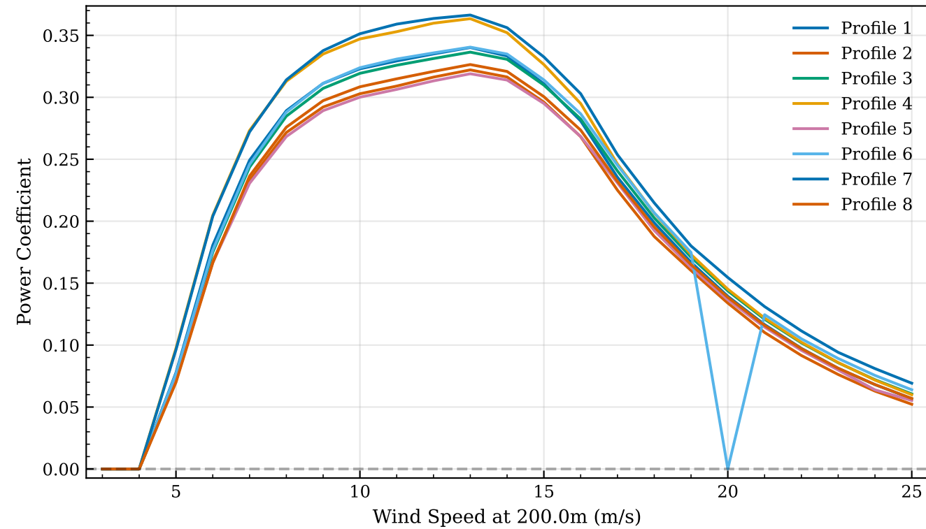
Power Coefficient
