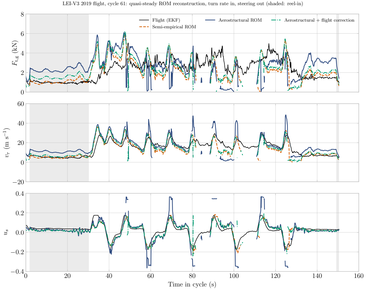
Figure 5: As Fig. 4 for cycle 61.
