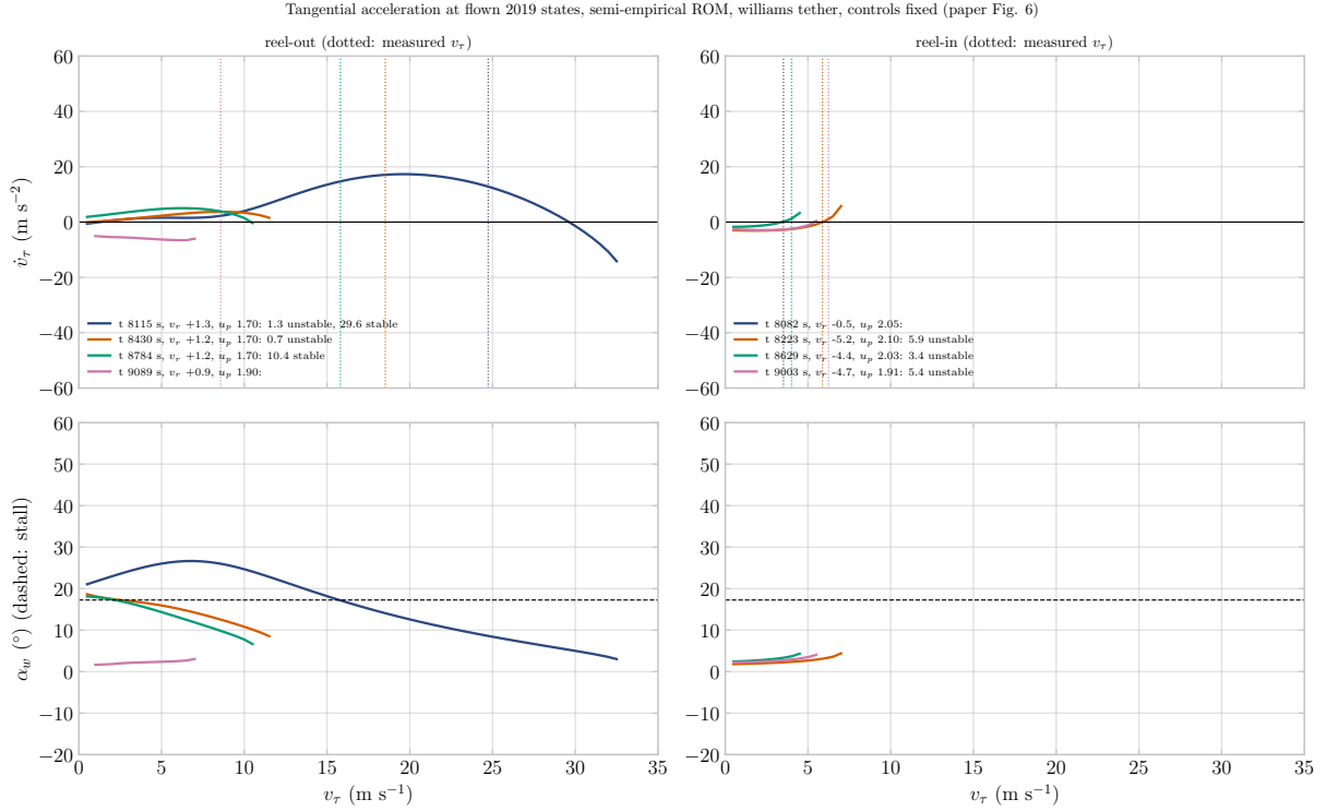
Figure 11: As Fig. 10 with the Williams tether: the radial row and the ground closure are solved at each speed for the kite-end tension, the tether length and the last element's angles. The reel-in fold remains.
