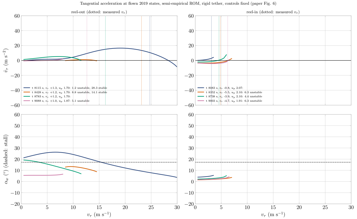
Figure 10: Tangential acceleration and wing angle of attack against tangential speed at flown 2019 states (semi-empirical ROM, controls fixed, tension from the radial balance). Reel-in branches end at the fold of the radial balance.
