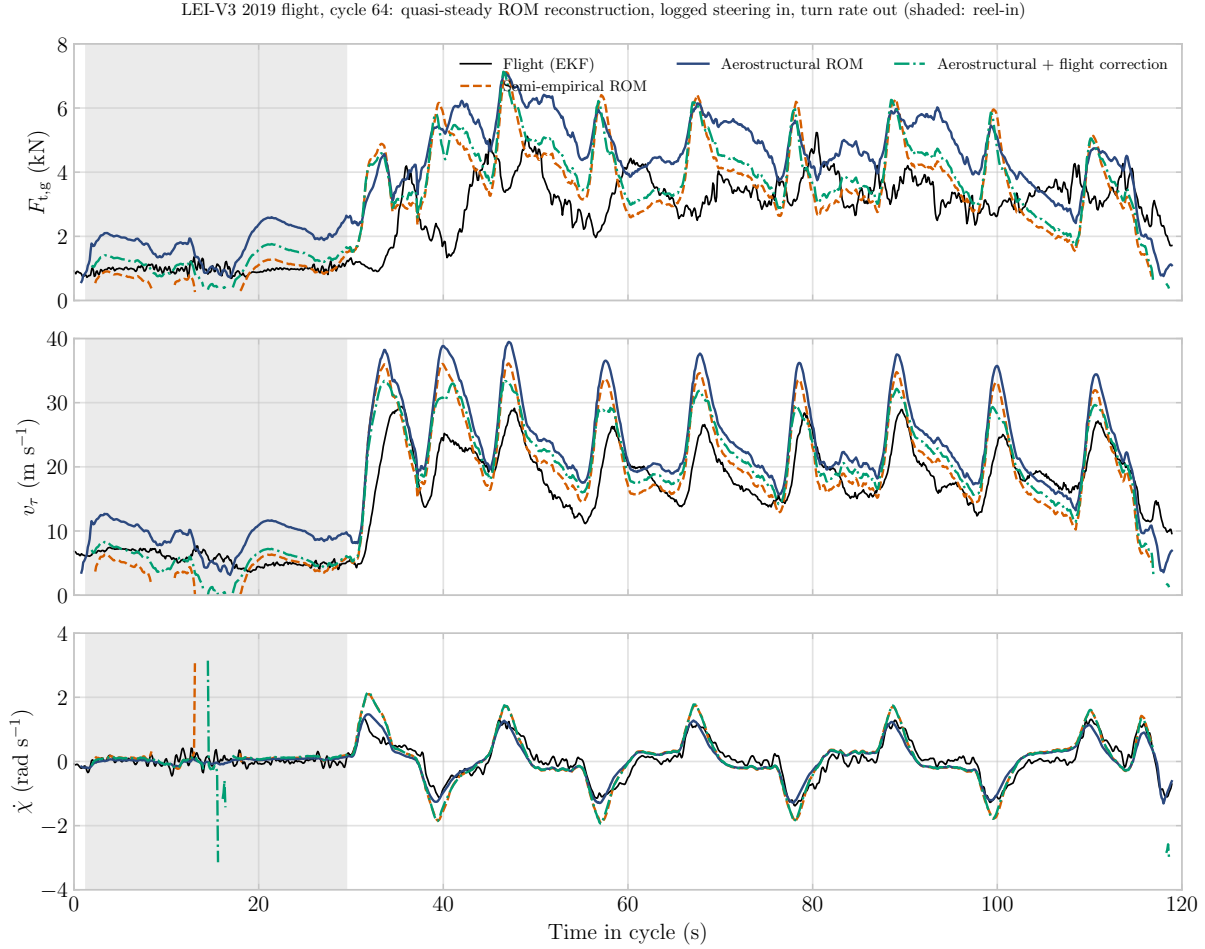
Figure 6: Cycle 64 with the logged steering as input.
