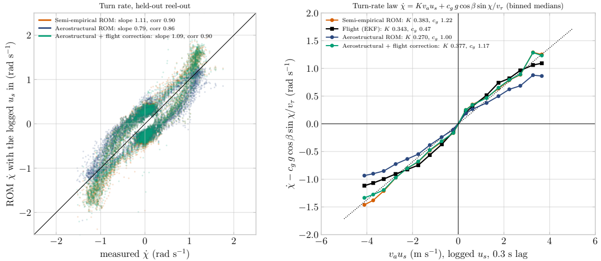
Figure 8: The turn rate of each ROM with the logged steering as input against the measured one (left, held-out reel-out samples), and the turn-rate law with the gravity term removed, binned in v_a u_s (right): the flight against the ROMs. The tuned ROMs sit on the flight’s K within 10 %; the aerostructural gain under-turns by a third. The flight’s response bends below linear beyond |v_a u_s| \approx 3 , a saturation at full steering that a linear gain cannot follow, which is where the tuned ROMs’ peak turn rates overshoot.
