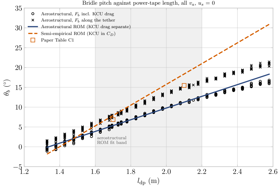
Figure 3: Bridle pitch against power-tape length: coupled trims measured against the bridle resultant ( \theta_b ) and against the tether direction, the aerostructural relation and the semi-empirical one.
