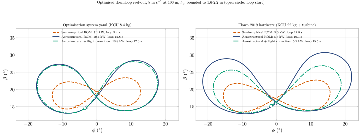
Figure 9: The optimised loops in azimuth and elevation, per ROM and hardware.
