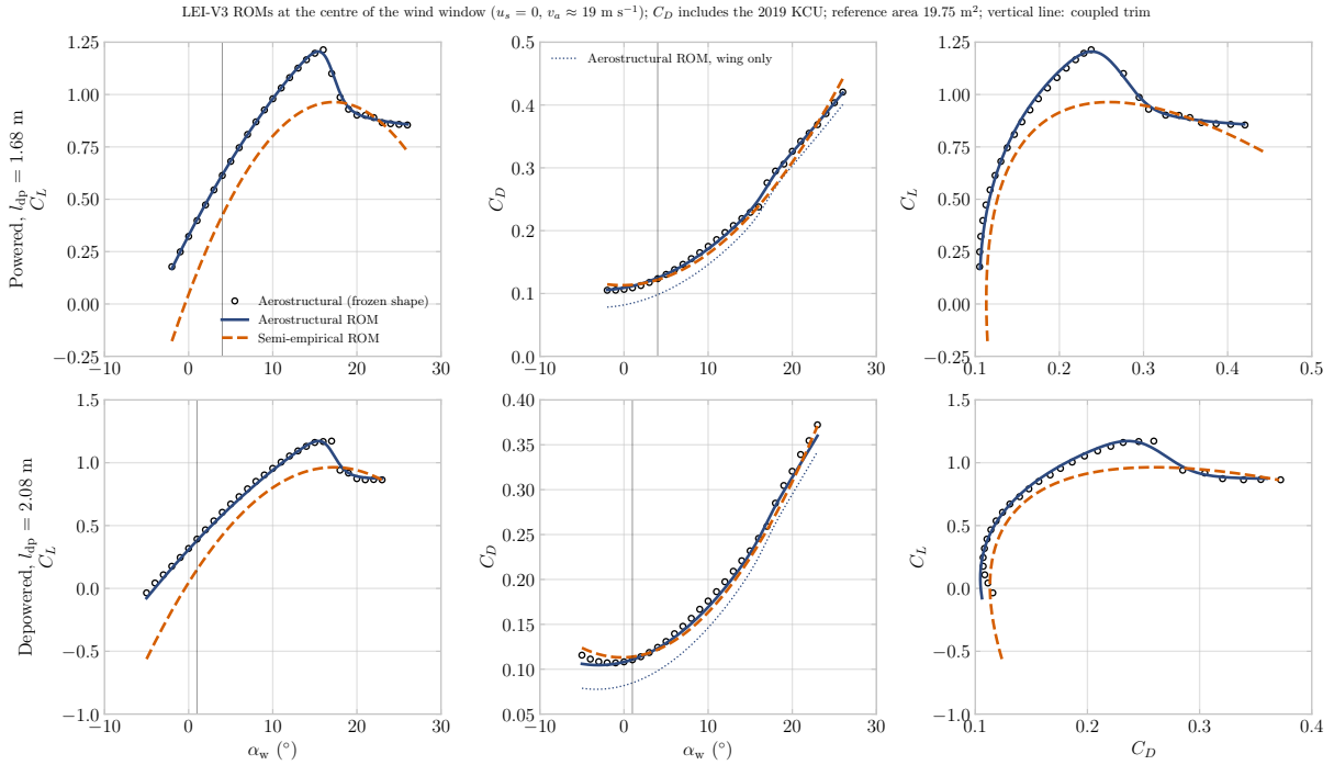
Figure 2: Lift and drag polars at the powered and depowered setting ( u_s = 0 , v_a \approx 19 \text{ m s}^{-1} , C_D with the 2019 KCU): coupled frozen-shape data, the aerostructural ROM and the semi-empirical ROM.
