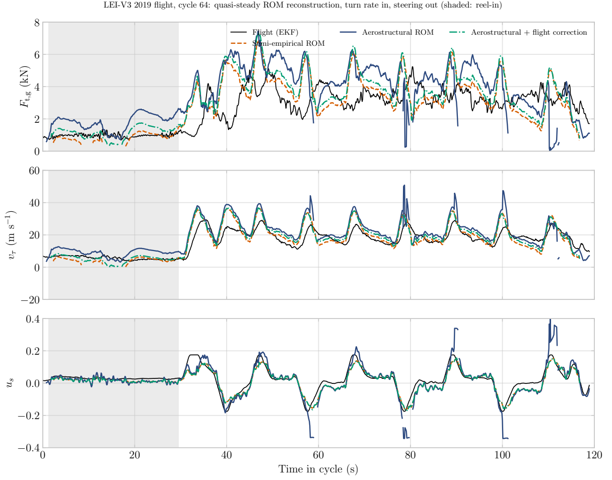
Figure 4: Cycle 64 (held out) with the measured turn rate as input and the steering solved: ground tension, tangential speed and the steering each ROM needs, against the EKF reconstruction (solid black, logged u_s with the rig's zero offset). Shaded: reel-in. Gaps are samples without a converged root.
