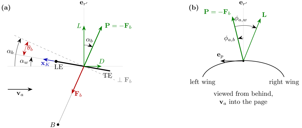
Figure 1: Geometric definitions (angles exaggerated). (a) Side view in the wing's symmetry plane: centre-panel chord with axis \mathbf{x}_K , apparent wind \mathbf{v}_a , the wing's lift and drag, the bridle resultant \mathbf{F}_b acting on the wing from the bridle point B and its reverse \mathbf{P} (collinear with \mathbf{F}_w for a massless kite). \alpha_w is the chord angle from the oncoming flow, \alpha_b the angle of the line perpendicular to \mathbf{F}_b (equally, of \mathbf{P} from \mathbf{e}_{r'} ), and \theta_b = \alpha_b - \alpha_w the bridle pitch fixed by the bridle geometry and depower setting. (b) Rear view about \mathbf{v}_a : the bridle roll \phi_{a,b} of \mathbf{P} and the steering roll \phi_{a,w} of the lift relative to it, both measured positive toward the left wing; drawn for u_s > 0 (right turn, \phi_{a,w} < 0 ).
