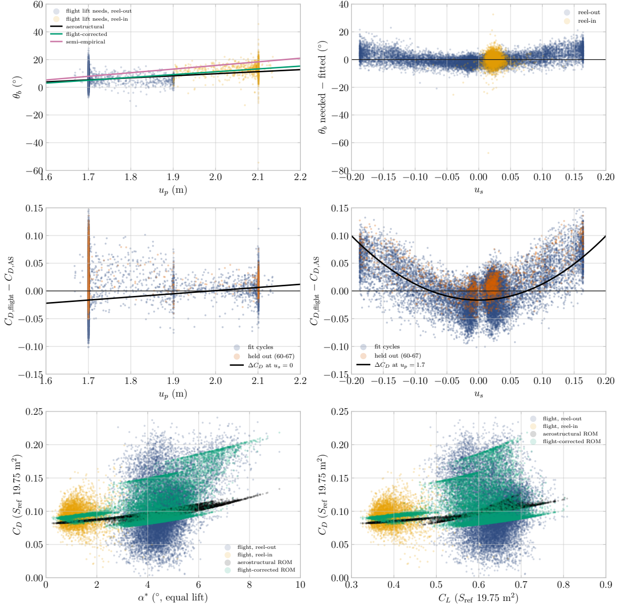
Figure 7: Steps 1–2 on the 2019 flight. Top: the \theta_b the flight lift needs against u_p , with the aerostructural, flight-corrected (steps 1–2) and semi-empirical relations, and its residual against steering. Middle: the drag polar at equal lift against u_p and u_s , fit and held-out cycles. Bottom: drag against \alpha^* and the drag polar.
