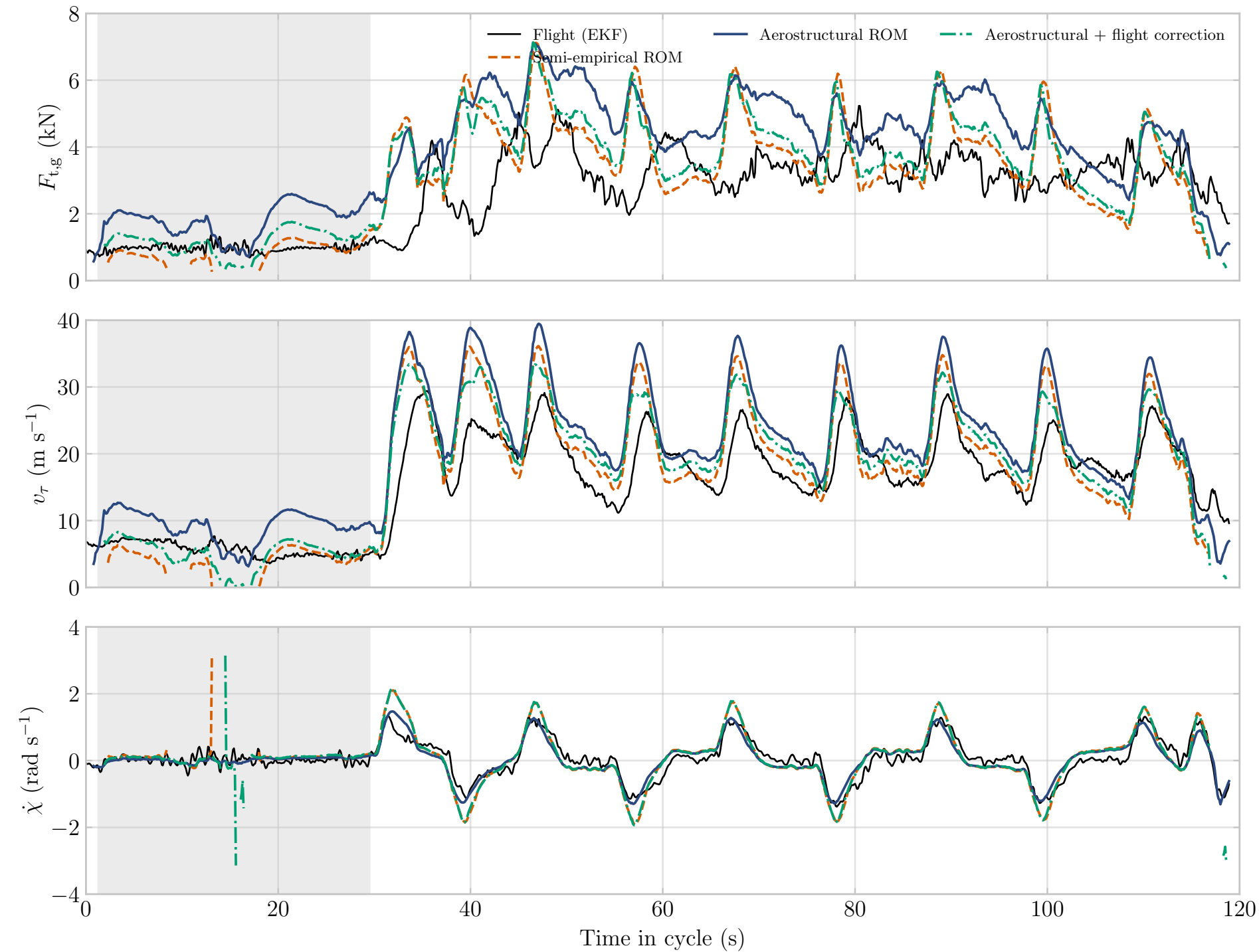
LEI-V3 2019 flight, cycle 64: quasi-steady ROM reconstruction, logged steering in, turn rate out (shaded: reel-in)
