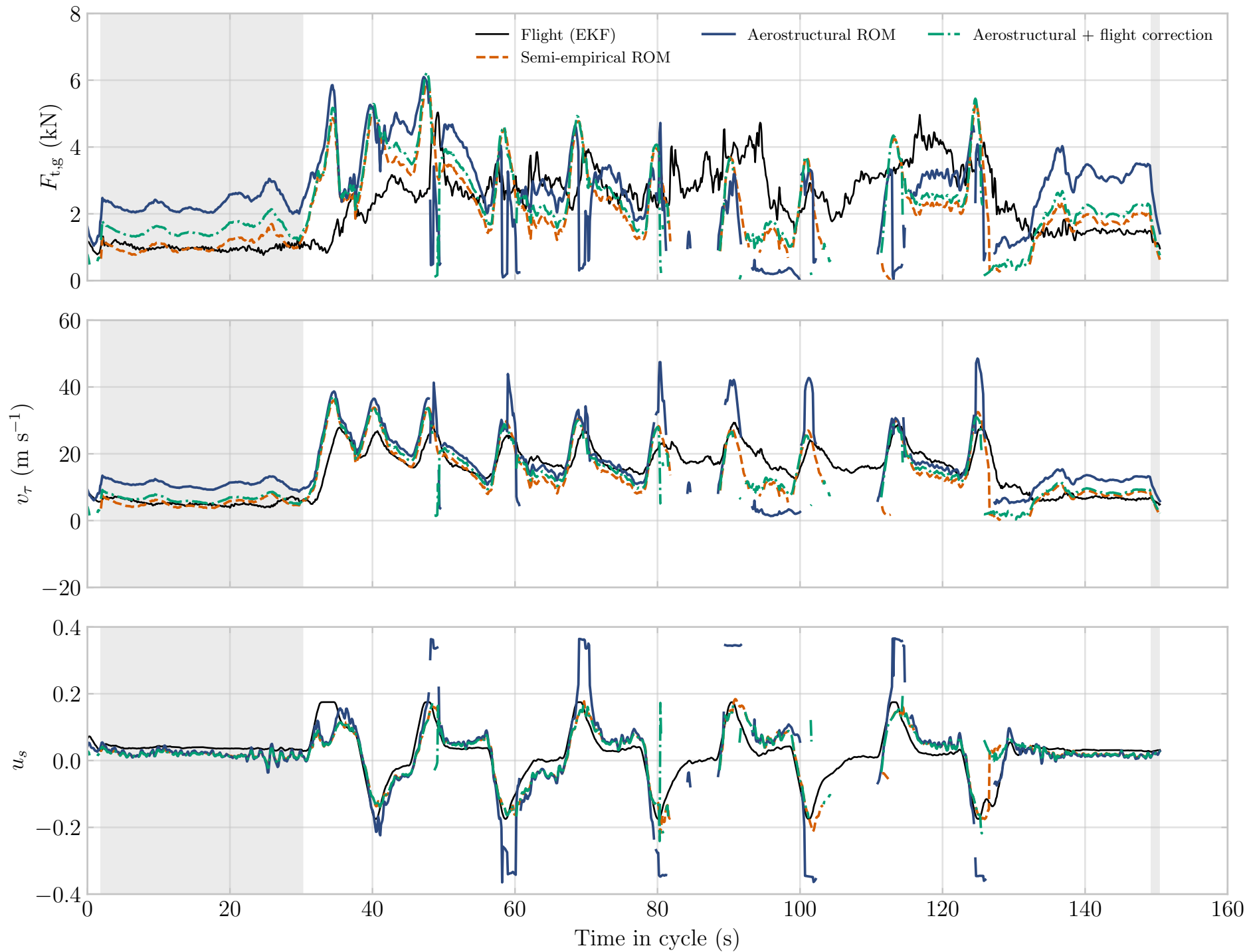
LEI-V3 2019 flight, cycle 61: quasi-steady ROM reconstruction, turn rate in, steering out (shaded: reel-in)
