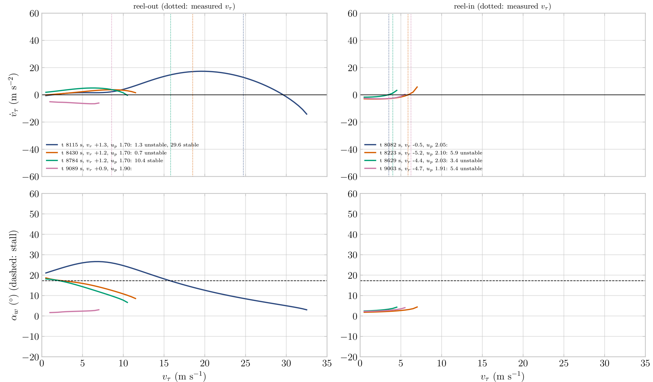
Tangential acceleration at flown 2019 states, semi-empirical ROM, williams tether, controls fixed (paper Fig. 6)
