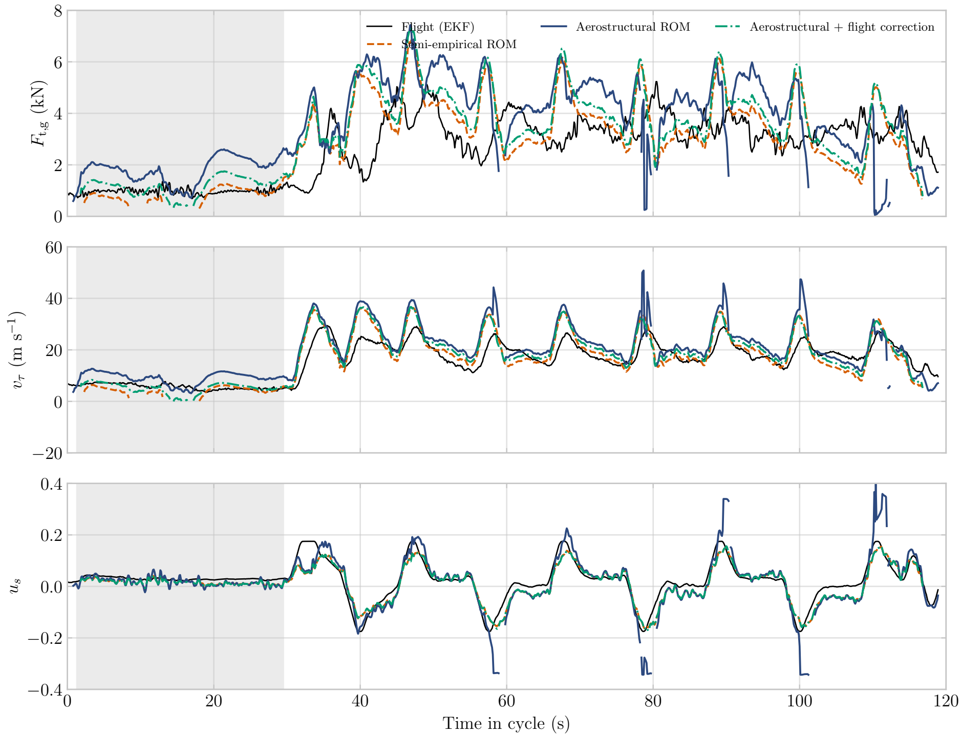
LEI-V3 2019 flight, cycle 64: quasi-steady ROM reconstruction, turn rate in, steering out (shaded: reel-in)
