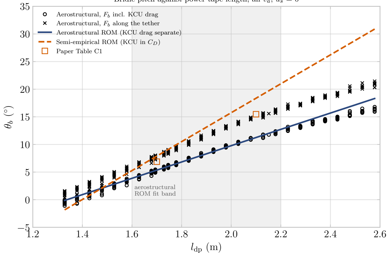
Bridle pitch against power-tape length, all v_a, u_s = 0
