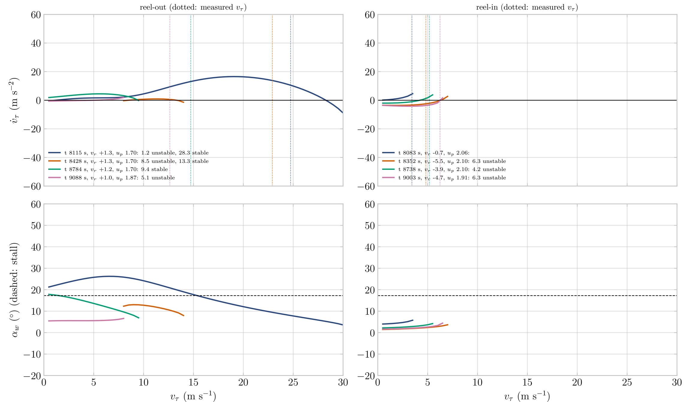
Tangential acceleration at flown 2019 states, semi-empirical ROM, rigid tether, controls fixed (paper Fig. 6)
