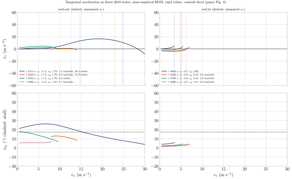
Figure 8: Tangential acceleration and wing angle of attack against tangential speed at flown 2019 states (semi-empirical ROM, controls fixed, tension from the radial balance). Reel-in branches end at the fold of the radial balance.
