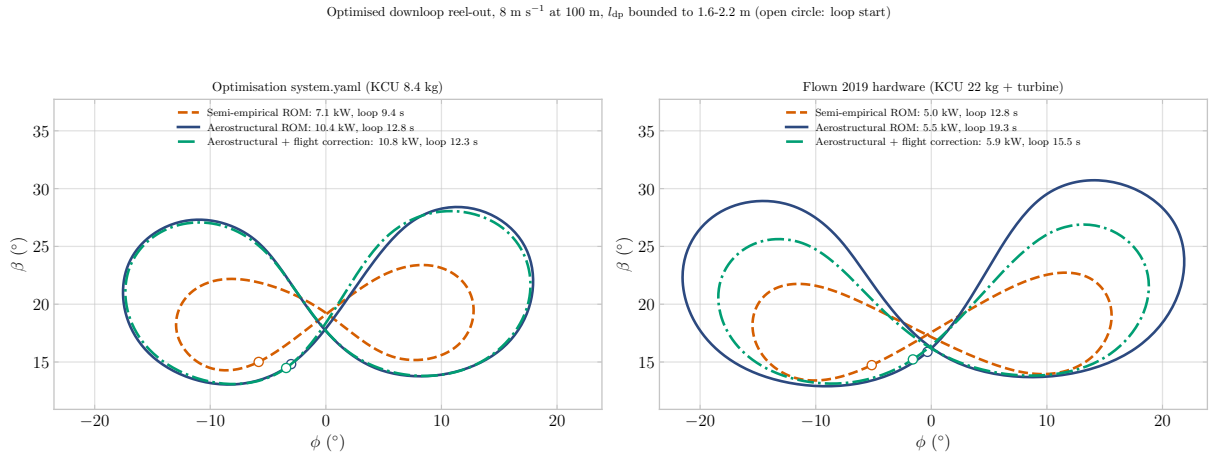
Figure 7: The optimised loops in azimuth and elevation, per ROM and hardware.
