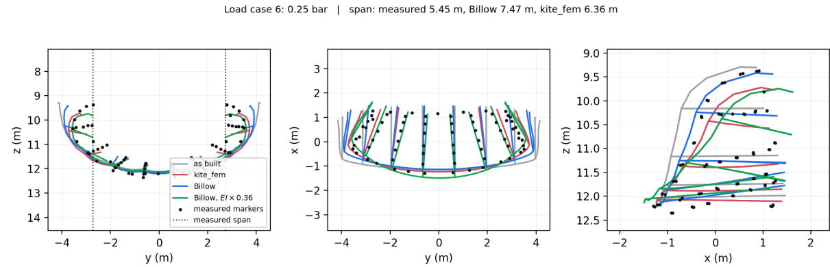
Figure 14: Load case 6.
