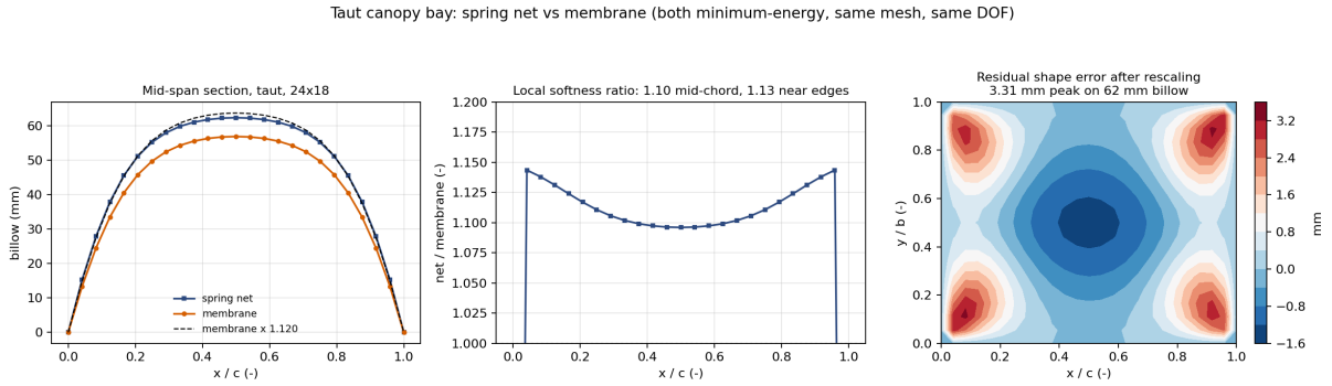
Figure 24: Taut bay, 24 \times 18 , both minimised on the same mesh with the same 1425 degrees of freedom, so this is purely the canopy model. The net billows 9.6% deeper; the best single scale factor is 1.120, and a 3.31 mm residual shape difference remains after removing it.
