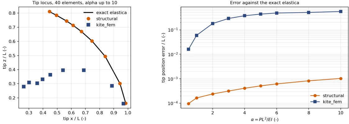
Figure 1: Tip locus and error against the exact elastica, 40 elements. Billow tracks the exact curve across the whole range; kite_fem departs progressively and its tip deflection saturates beyond \alpha \approx 2 .
