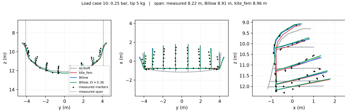
Figure 18: Load case 10.
