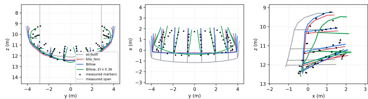
Figure 16: Load case 8.
