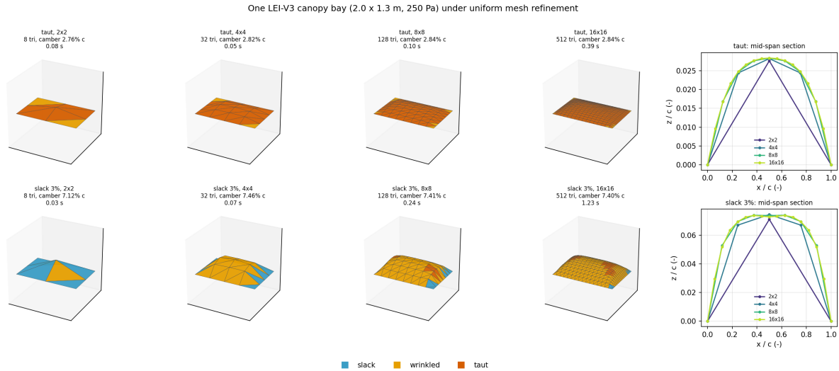
Figure 25: One bay under uniform refinement. A 2 \times 2 bay is a tent, not a canopy: the camber is only 2.8% low but the section is two straight lines. By 8 \times 8 the profile is visually converged.
