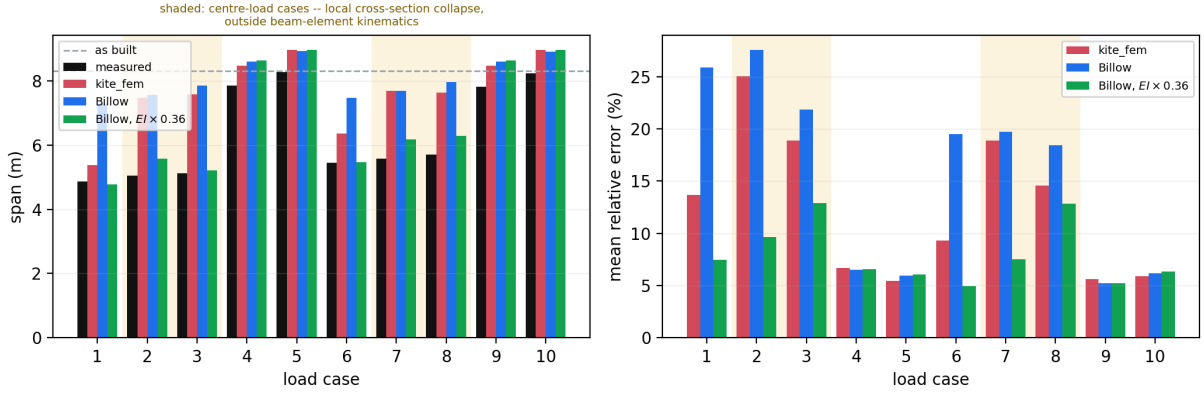
Figure 5: Span and mean relative error across the ten cases. Both codes overstate the span wherever they solve the physical branch; the gap is widest where gravity alone sets the shape and narrowest where an imposed tip load dominates. The shaded centre-load cases are reproduced by neither code, and are where Billow’s folded branch shows as a near-zero span.
