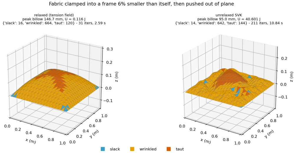
Figure 19: A panel clamped into a frame 6% smaller than itself, then pushed out of plane. The relaxed law converges in 31 iterations to a smooth billow; the unrelaxed one takes 211 and buckles into mesh-scale crumple at less than two-thirds the deflection.
