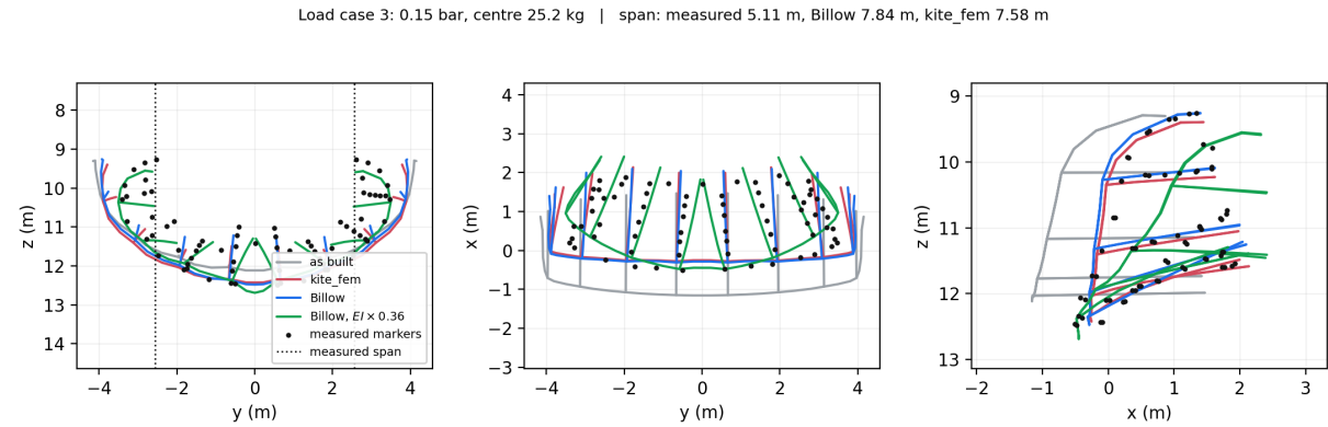
Figure 11: Load case 3.
