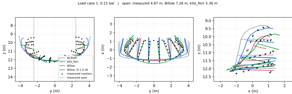
Figure 9: Load case 1.
