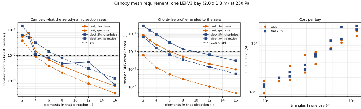
Figure 26: Camber and section-shape convergence, chordwise (solid) and spanwise (dashed), and cost per bay.
