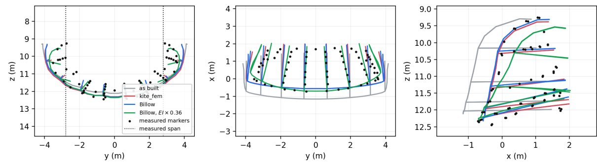
Figure 15: Load case 7.
