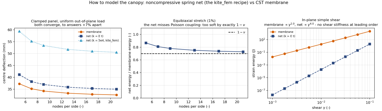
Figure 23: Spring net versus CST membrane on identical meshes, both minimised. Left: both converge under out-of-plane load, to answers 7% apart. Middle: under equibiaxial stretch the net is too soft by exactly 1 - \nu . Right: under in-plane shear the membrane energy scales as \gamma^{2.0} and the net as \gamma^{4.0} — the net has no shear stiffness at leading order .
