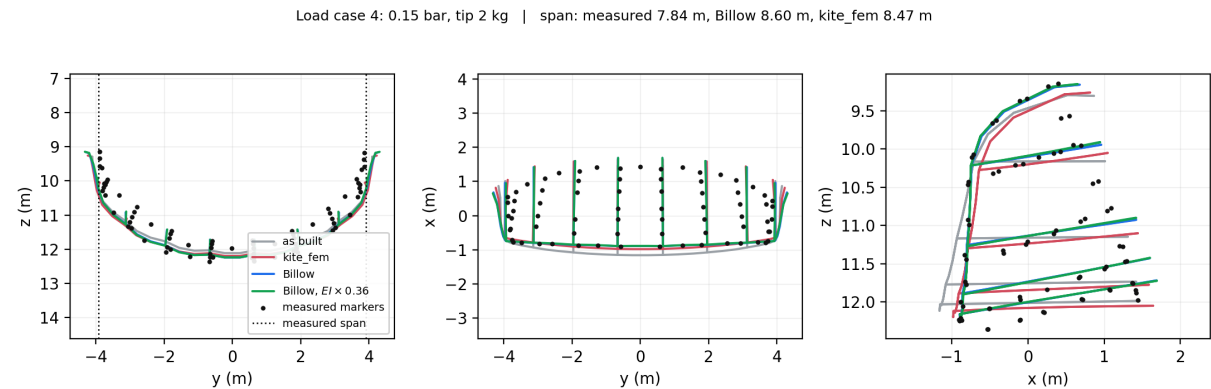
Figure 12: Load case 4.
