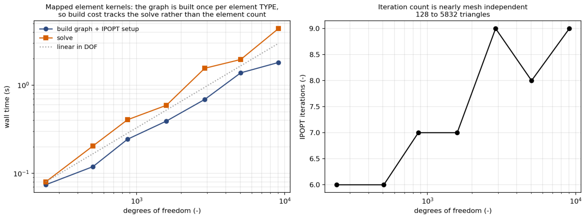
Figure 22: Build and solve time against problem size, and iteration count. Because the graph is built once per element type , build cost tracks the solve rather than the element count, and the iteration count is nearly mesh independent across a 37\times range in degrees of freedom.
