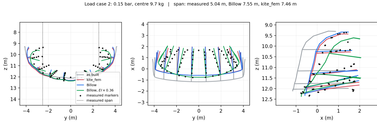
Figure 10: Load case 2.
