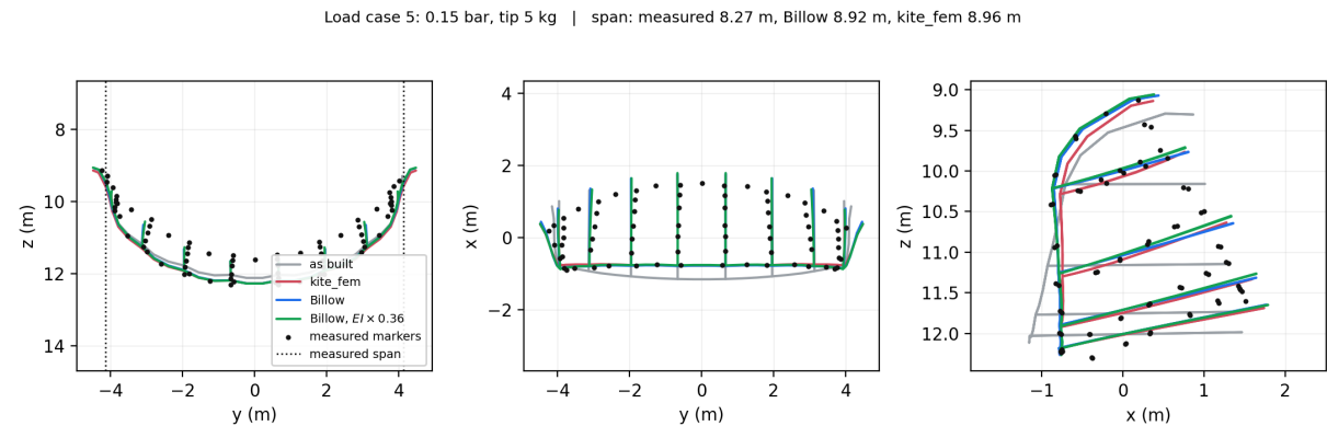
Figure 13: Load case 5.
