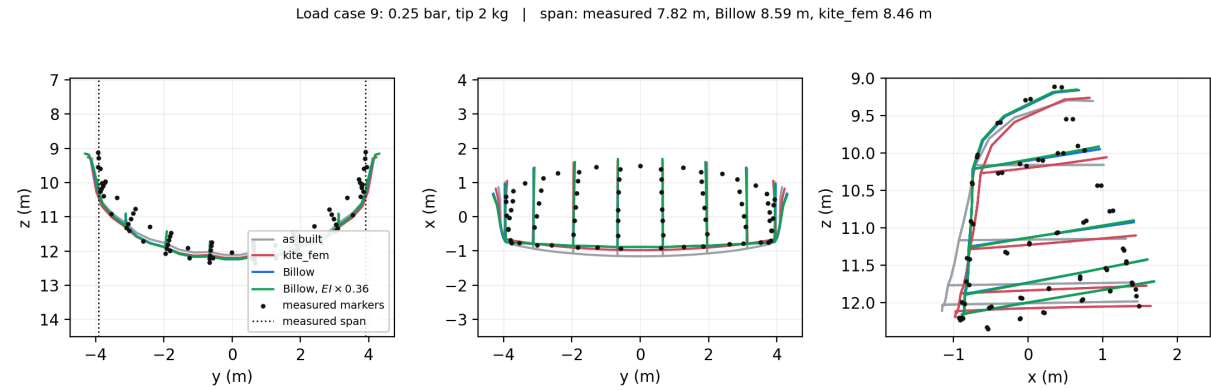
Figure 17: Load case 9.
