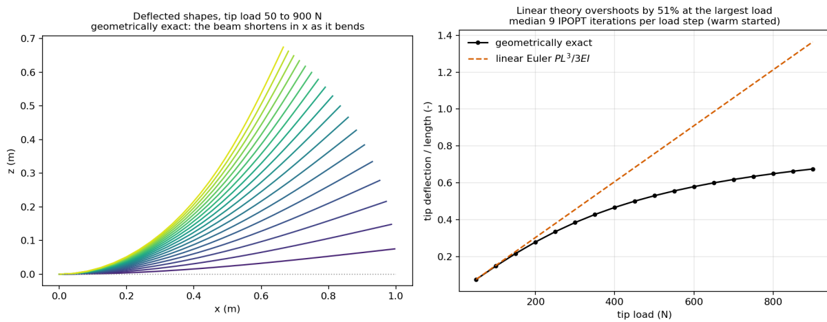
Figure 20: Deflected shapes under a tip load swept from 50 to 900 N, and tip deflection against linear theory. The beam visibly shortens in x as it bends — the geometric nonlinearity linear theory omits. At the largest load, linear theory overshoots by 51%.
