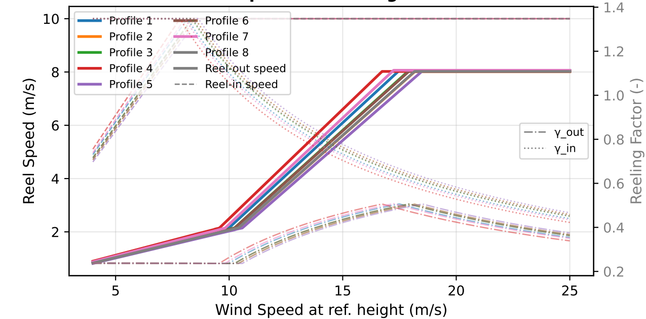
Reel Speeds & Reeling Factors
