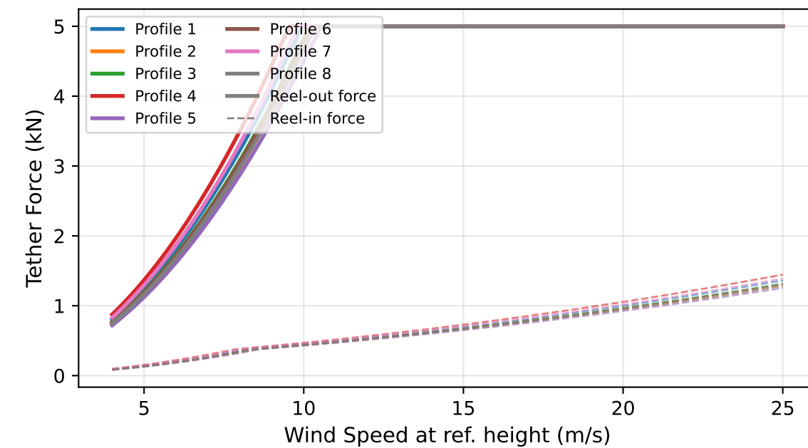
Tether Forces - All Profiles
