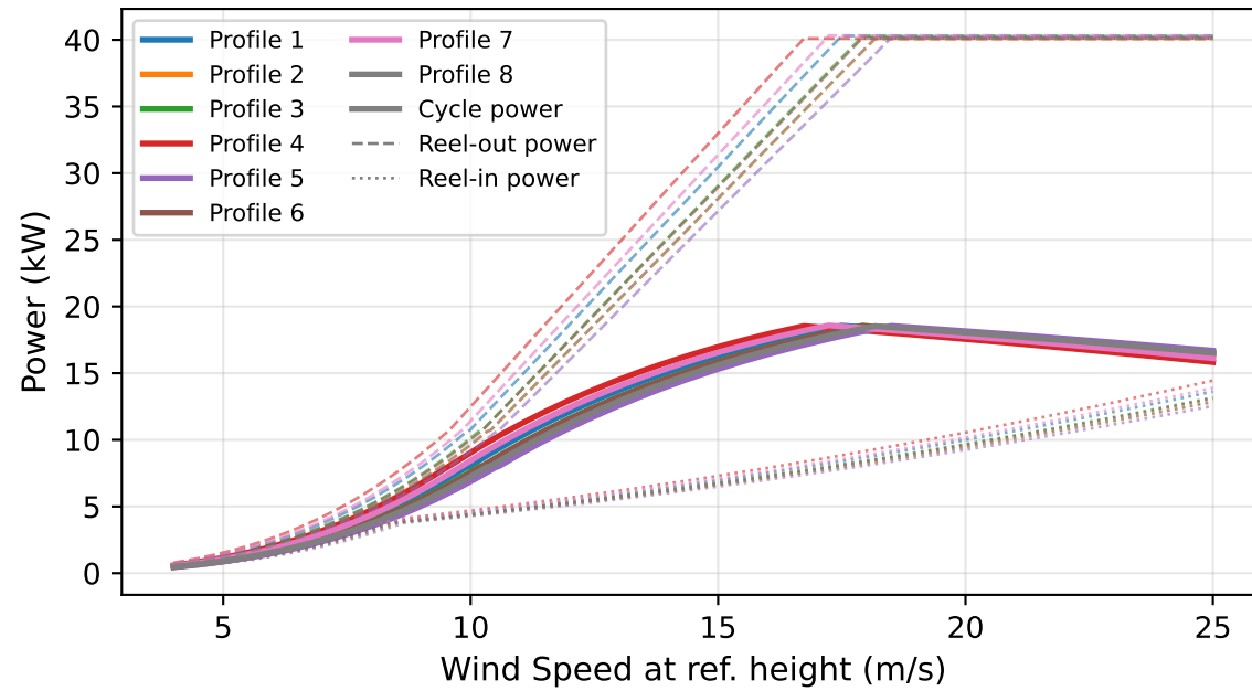
Power Output - All Profiles
