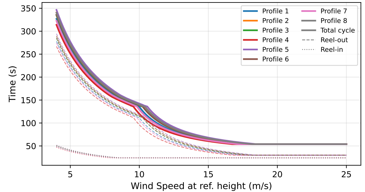
Cycle Times - All Profiles
