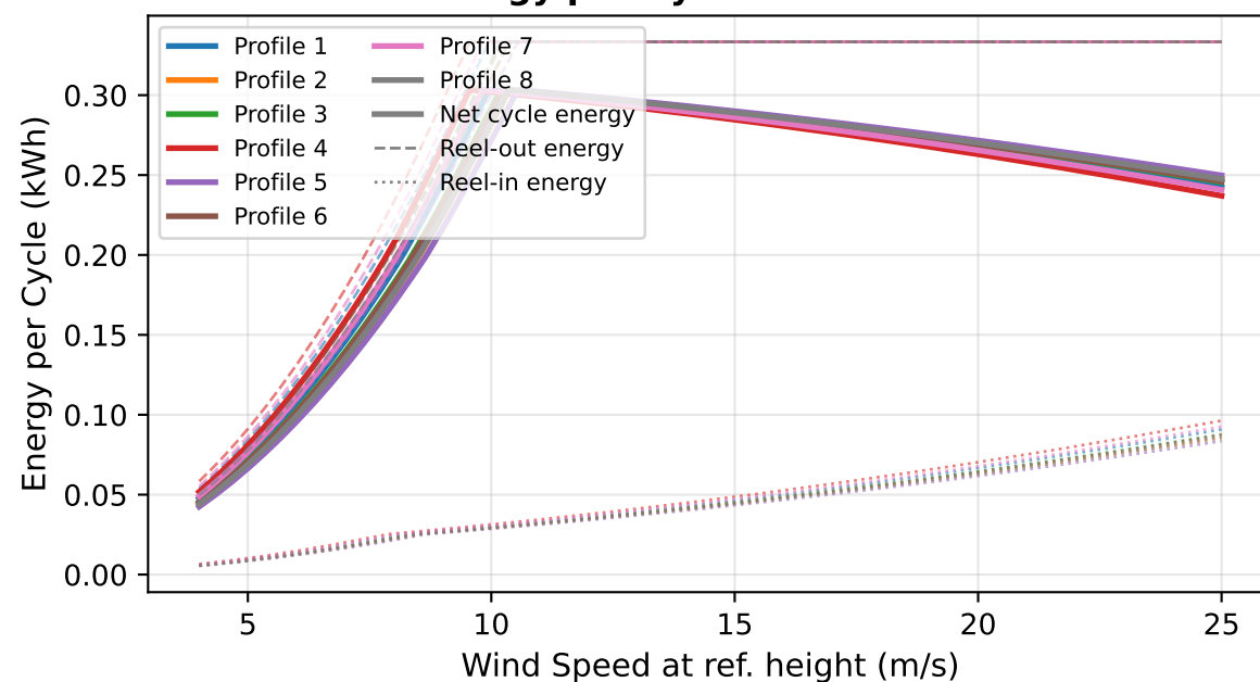
Energy per Cycle - All Profiles
