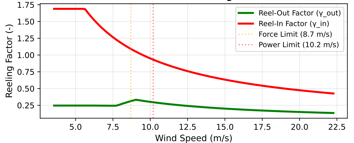
Dimensionless Reeling Factors
