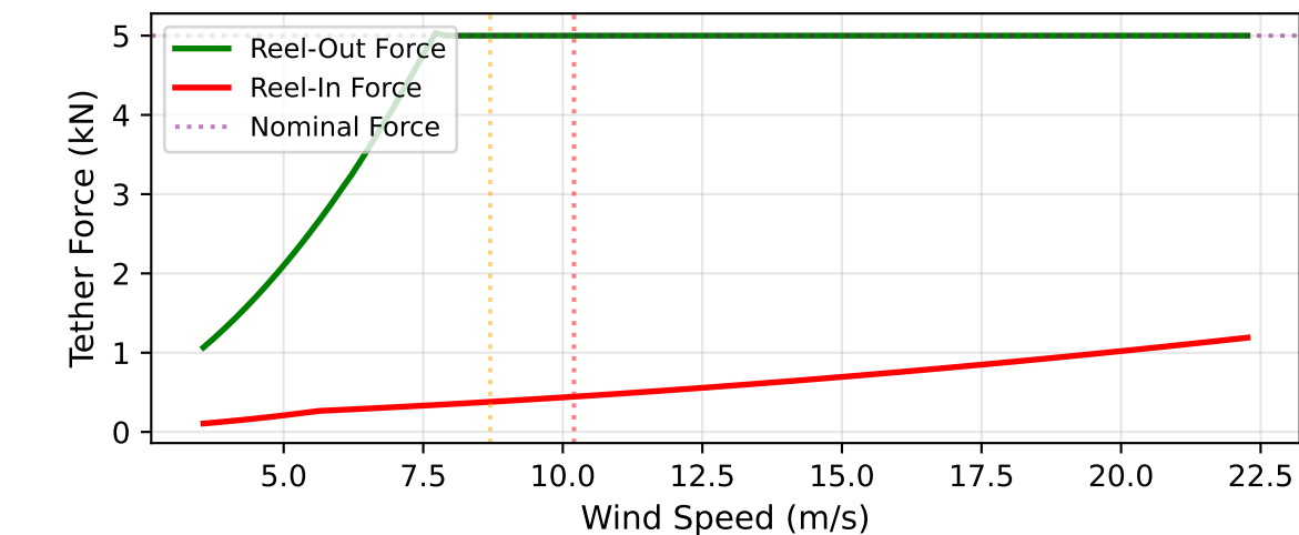
Tether Forces
