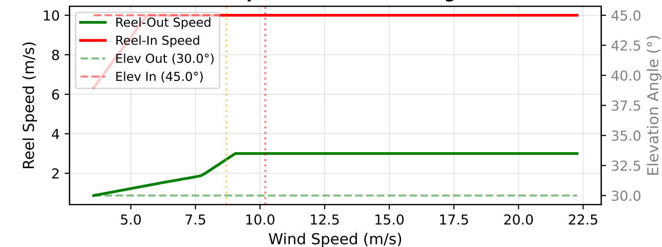
Reel Speeds & Elevation Angles
