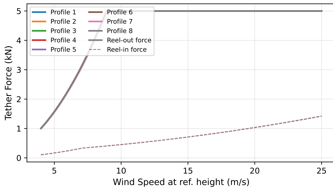
Tether Forces - All Profiles
