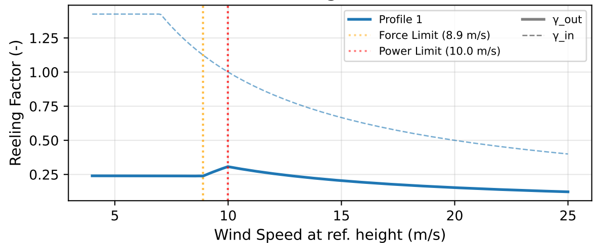
Dimensionless Reeling Factors - All Profiles
