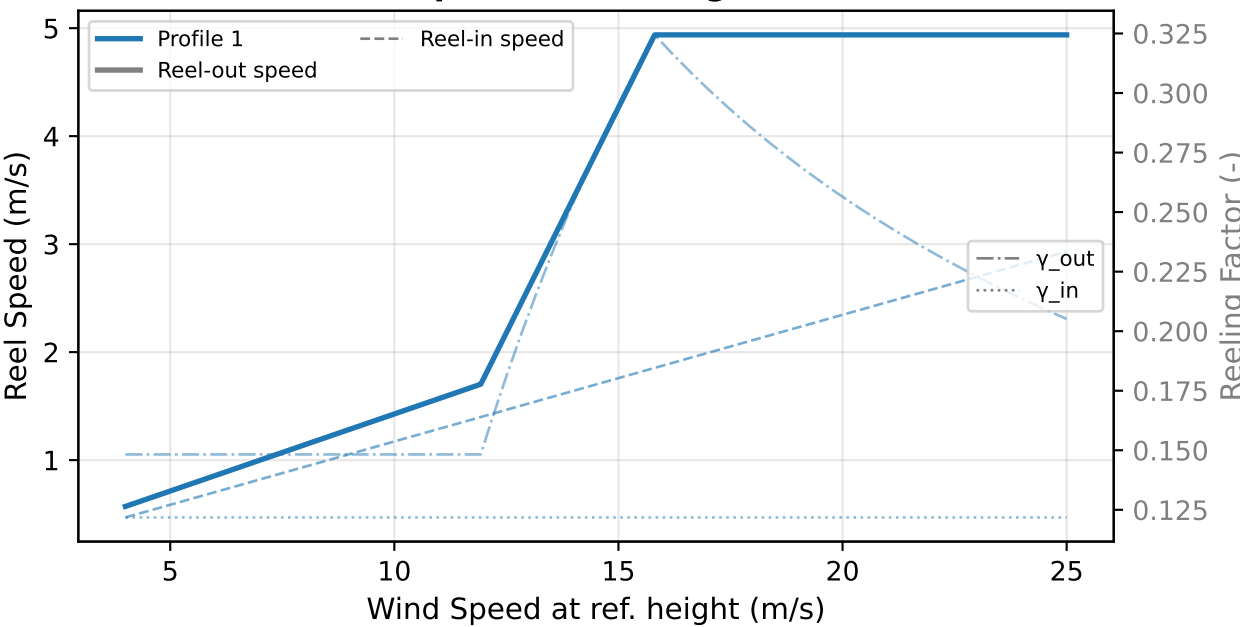
Reel Speeds & Reeling Factors
