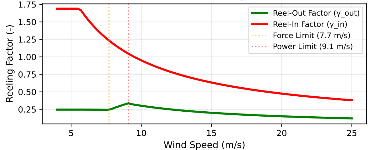
Dimensionless Reeling Factors
