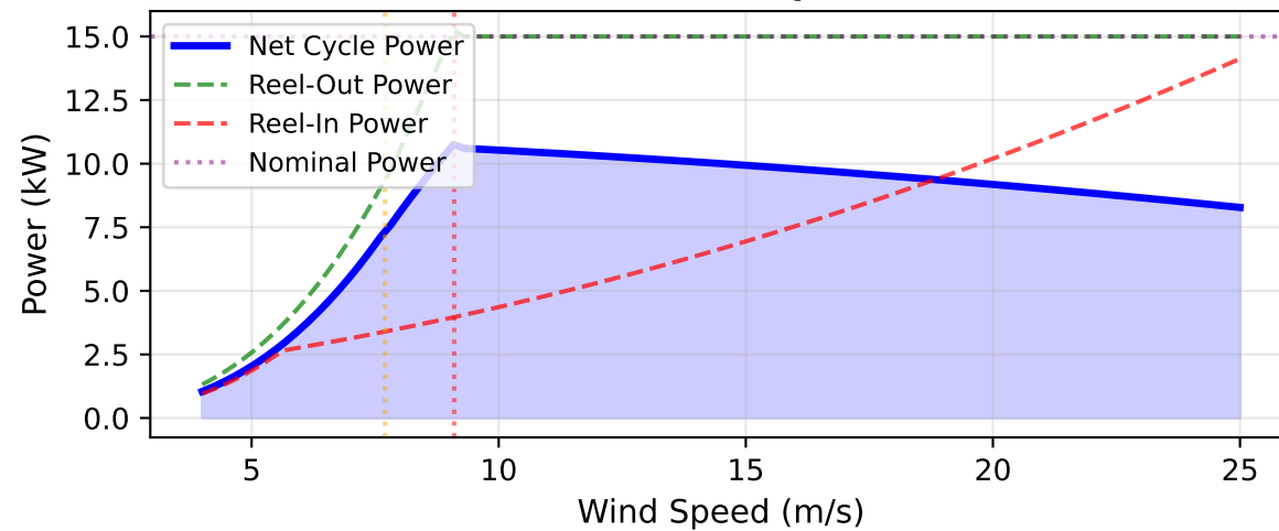
Power Output
