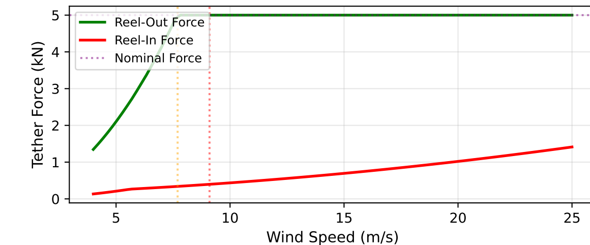
Tether Forces
