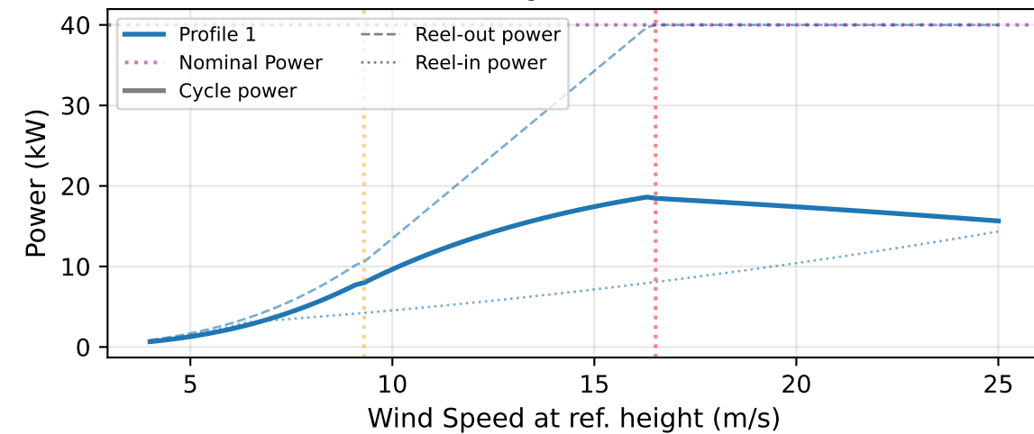
Power Output - All Profiles
