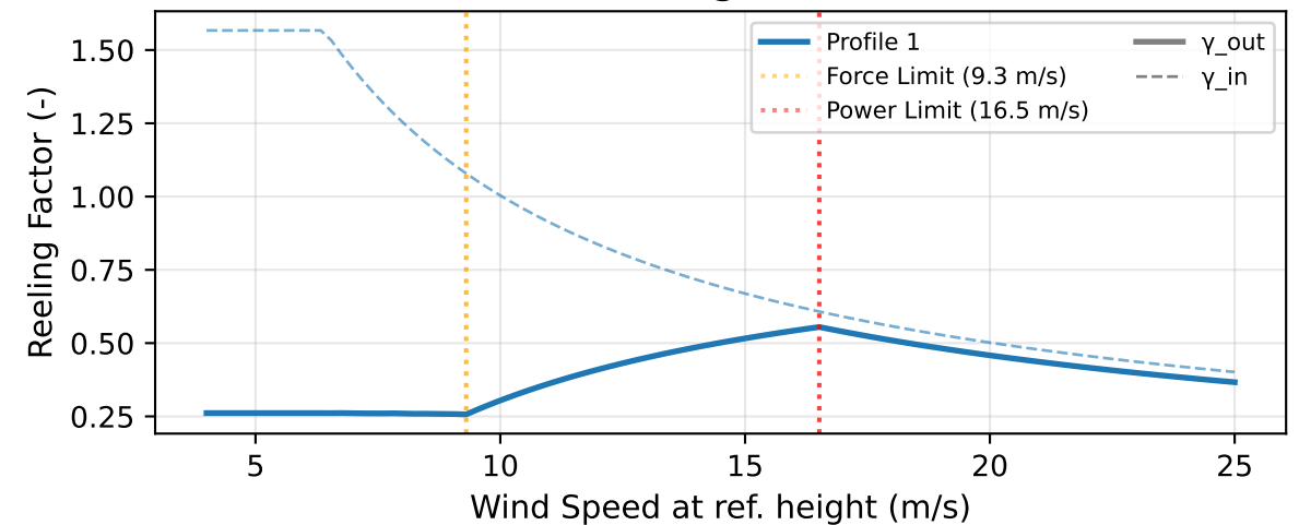
Dimensionless Reeling Factors - All Profiles
