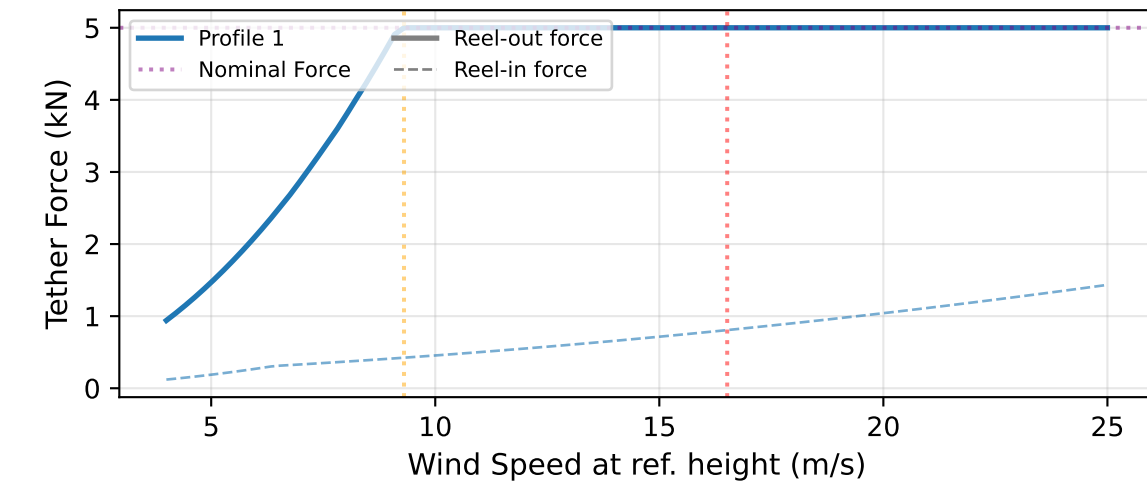
Tether Forces - All Profiles
