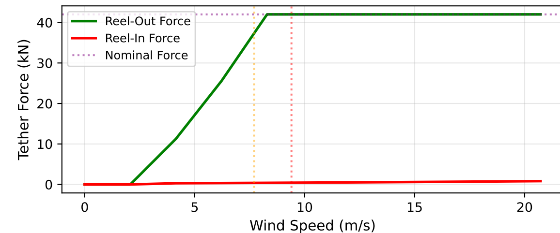
Tether Forces
