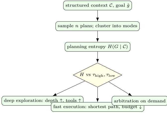
Fig. 2. Uncertainty-adaptive planning. Planning entropy selects one of three operating modes; verification failures trigger replanning rather than blind retry.
