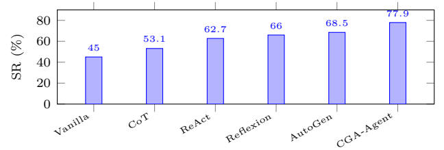
Fig. 4. Average task success rate of each method over the four datasets and three random seeds (values from Table V).
