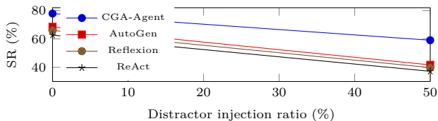
Fig. 8. Effect of distractor-document injection on task success rate (endpoints at 0% and 50% injection).
