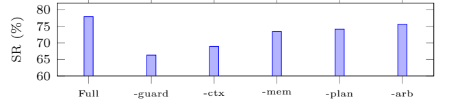
Fig. 7. Ablation: task success rate after removing each module, relative to the full model.
