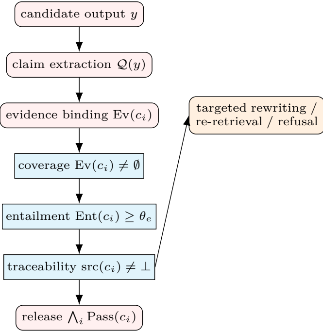
Fig. 3. The Claim-Evidence guardrail. Each claim must pass a coverage, an entailment and a traceability gate; failures are routed to targeted rewriting, re-retrieval or refusal.
