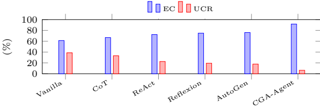
Fig. 5. Evidence coverage and unsupported-claim rate. The guardrail shifts the operating point far beyond what additional reasoning rounds achieve.
