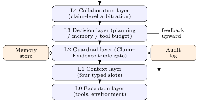
Fig. 1. Layered architecture of CGA-Agent. Data flows downward; control and verification feedback flow upward; the memory store and audit log are attached at the sides.
