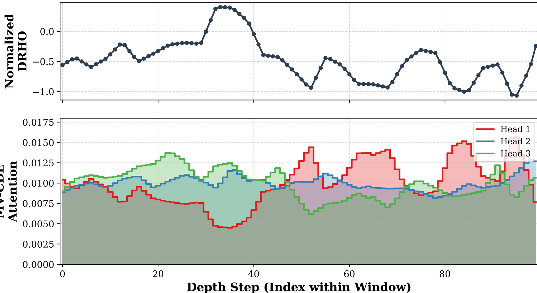
Attention Map (Feature: DRHO | Sample: 2)
