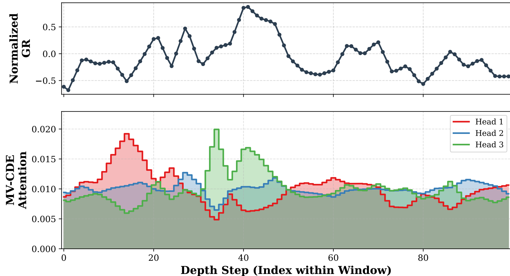
Attention Map (Feature: GR | Sample: 1)
