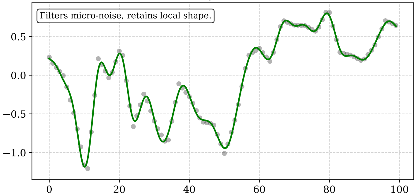
GP Smoothing (Narrow Kernel)
