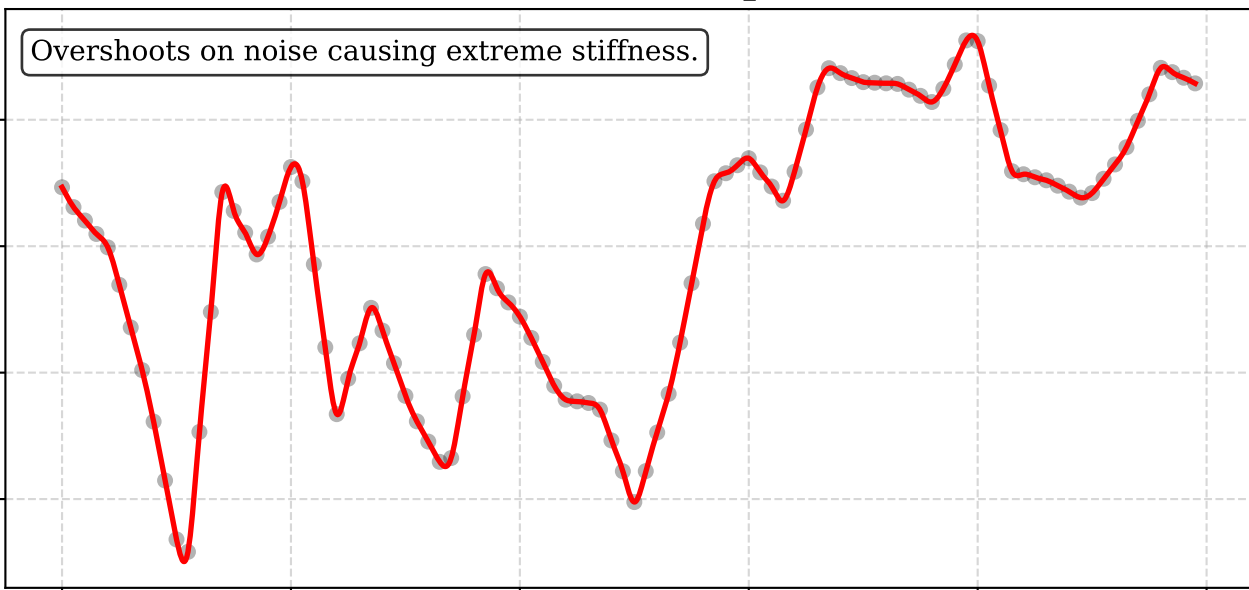
Natural Cubic Spline
