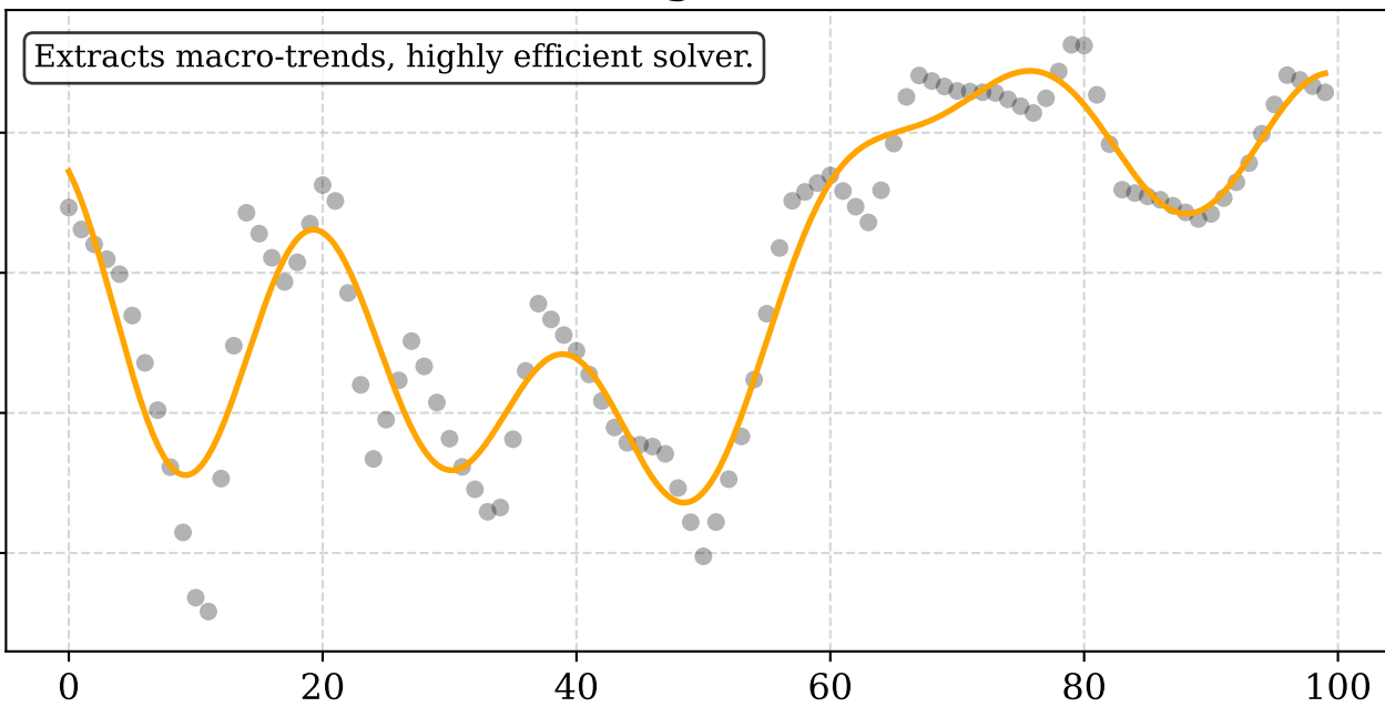
GP Smoothing (Wide Kernel)
