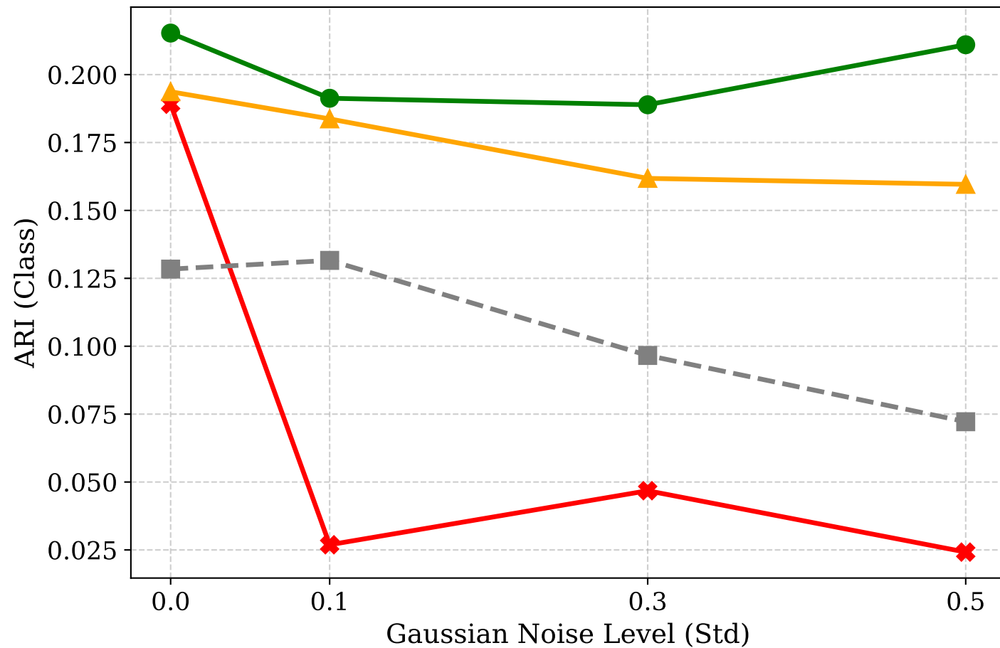
Classification Performance (ARI) ↓
