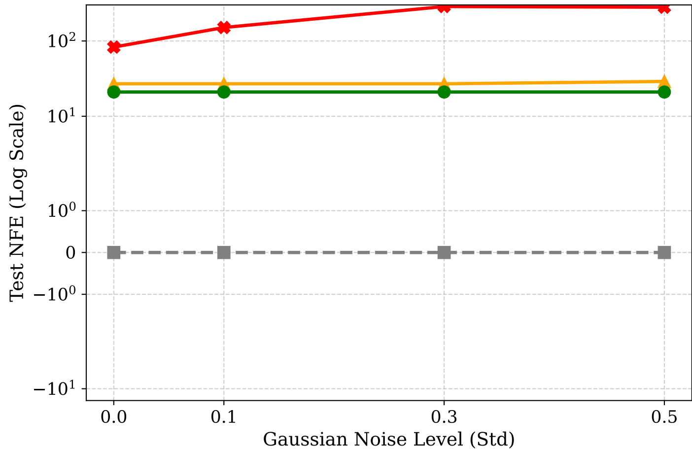
Computational Cost (Average NFE) ↑
