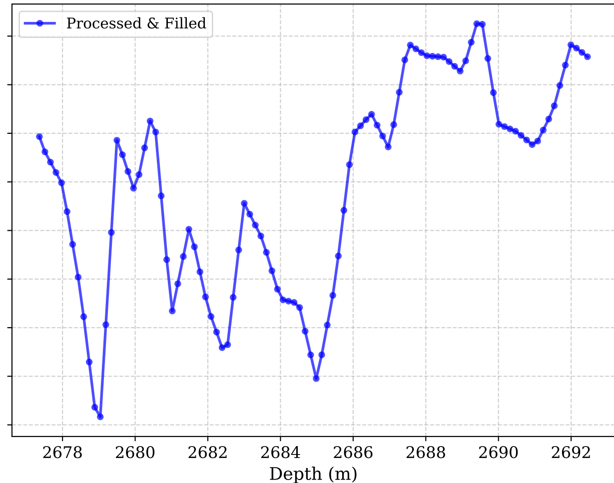
After: Processed Data for Neural CDE
