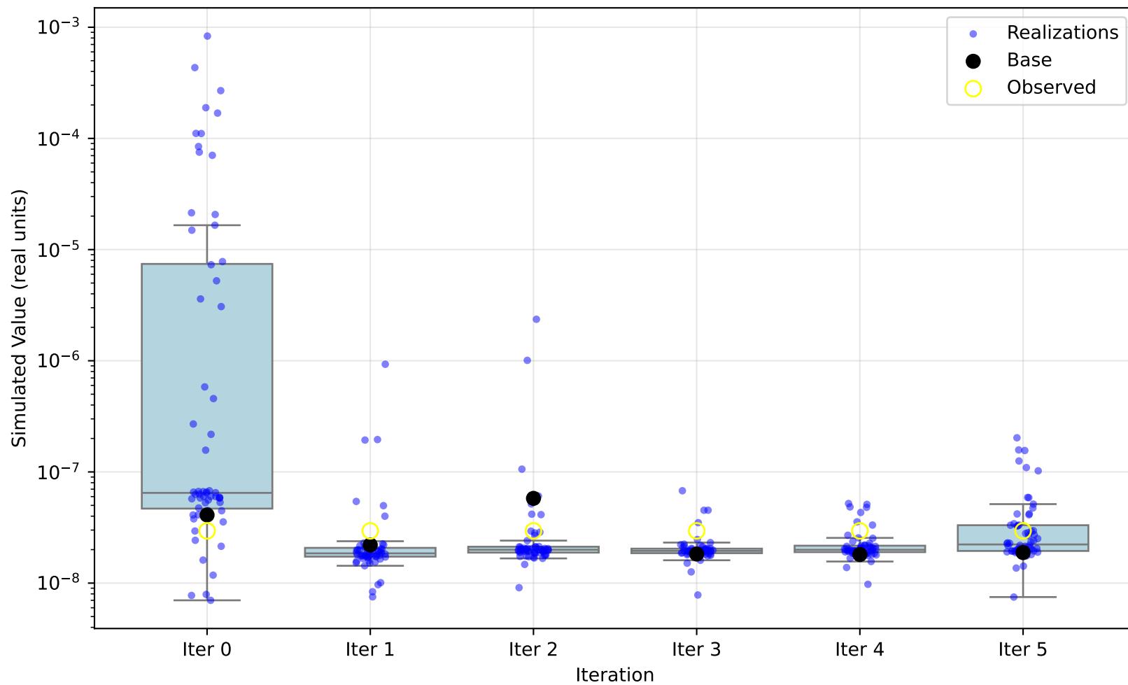
Simulated Ensemble vs Observed: al
