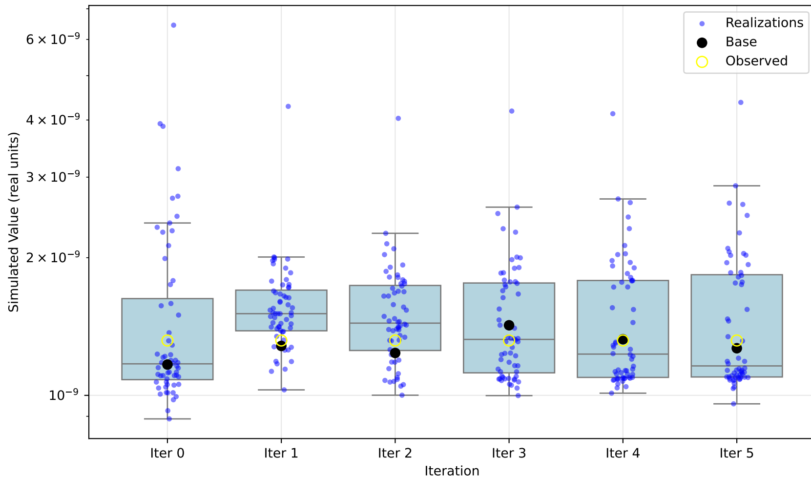
Simulated Ensemble vs Observed: as
