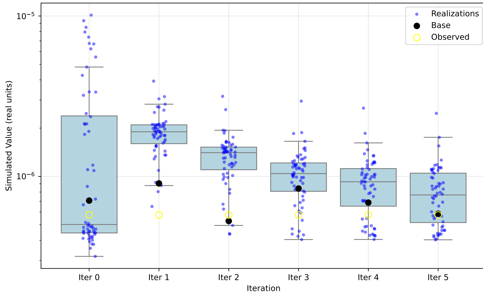
Simulated Ensemble vs Observed: ba
