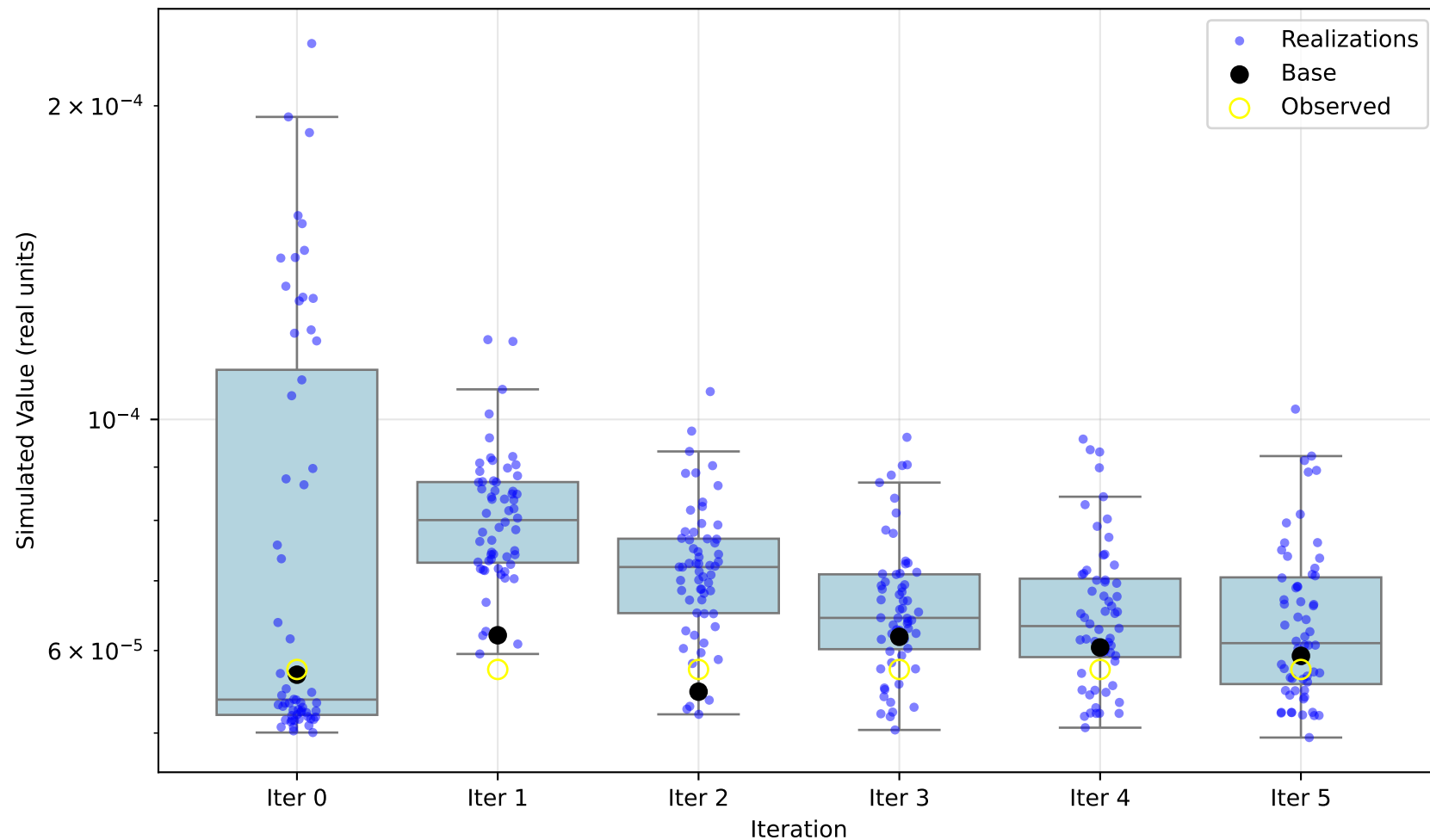
Simulated Ensemble vs Observed: cl
