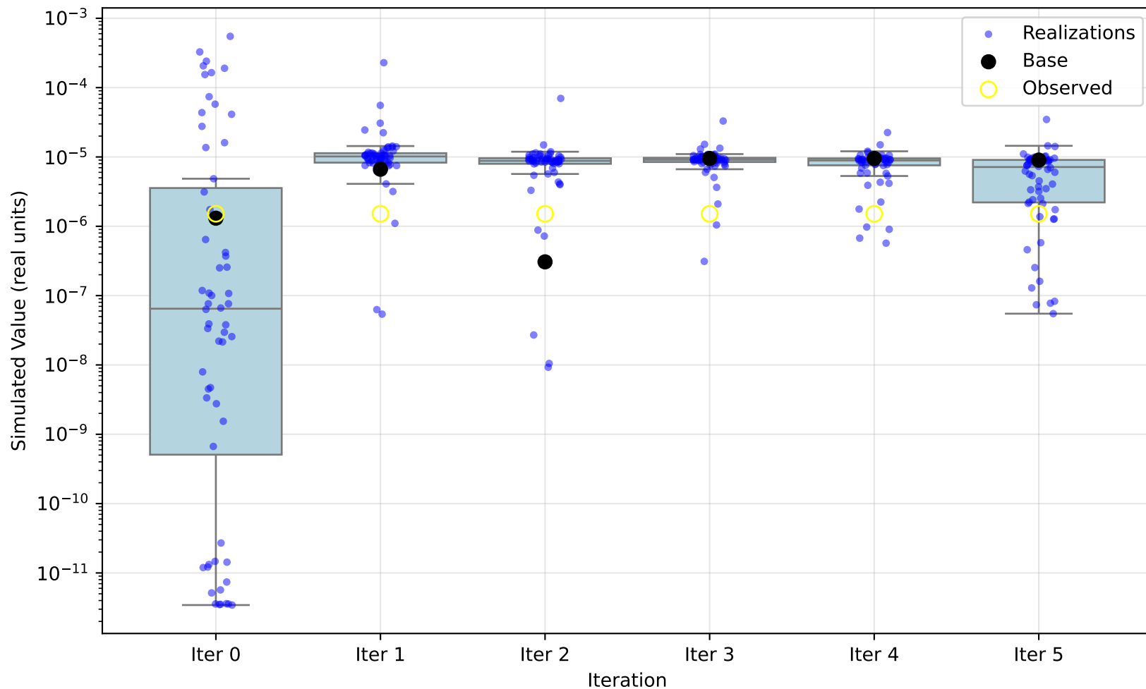
Simulated Ensemble vs Observed: fe
