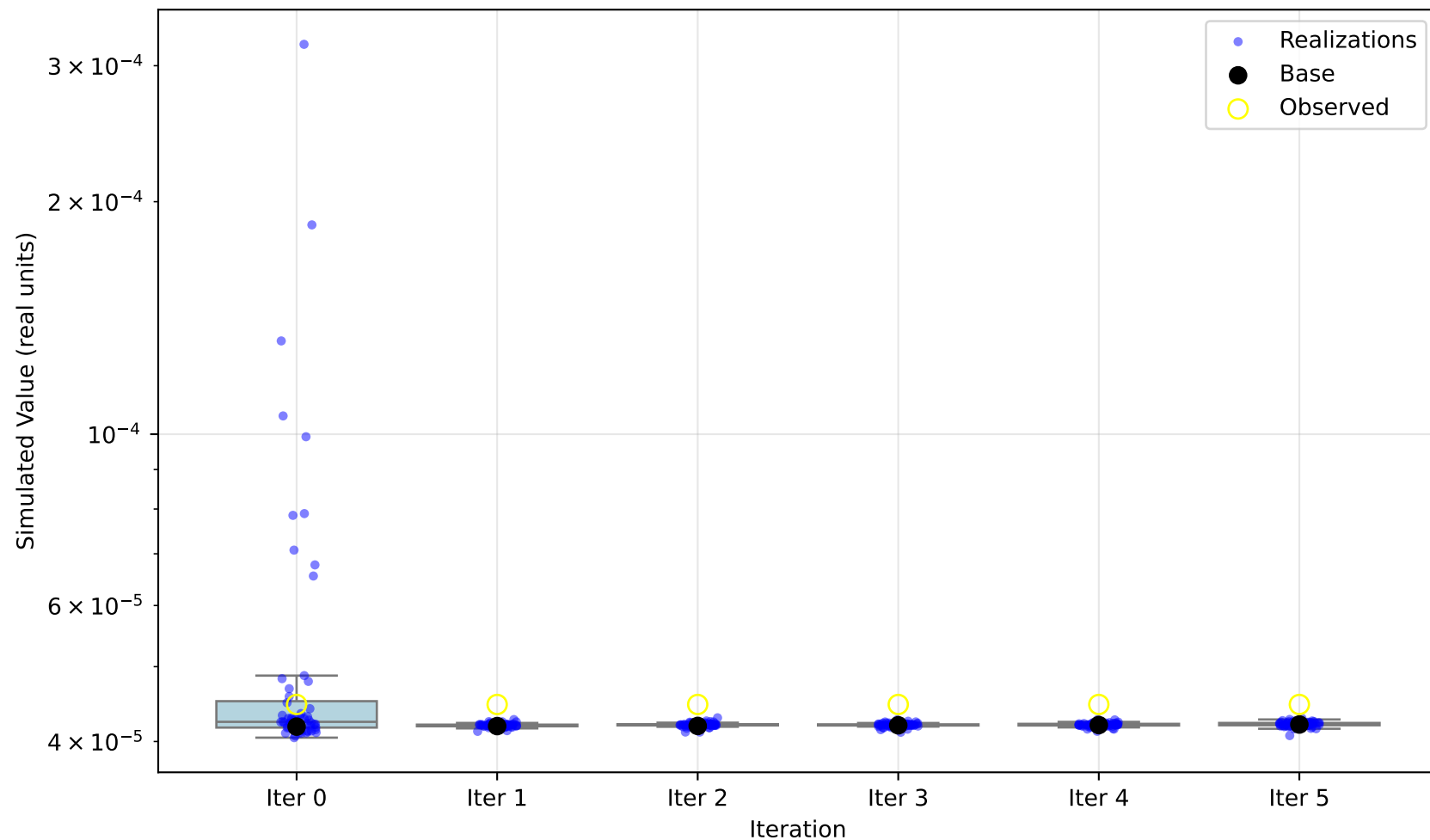
Simulated Ensemble vs Observed: k
