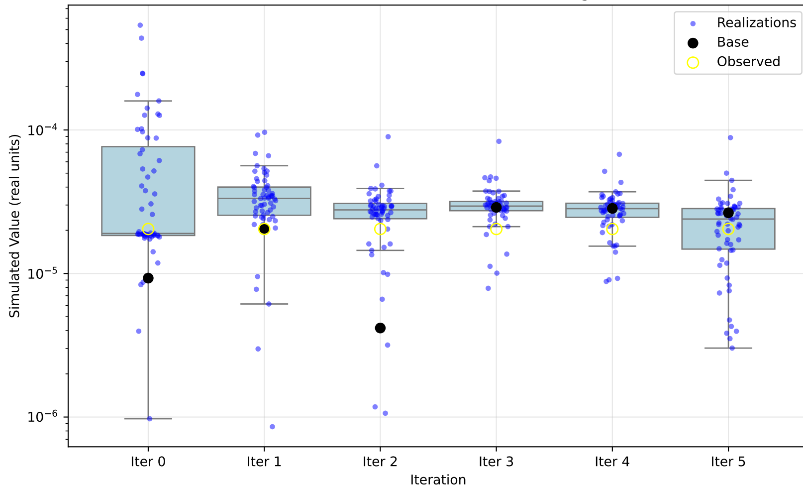
Simulated Ensemble vs Observed: mg
