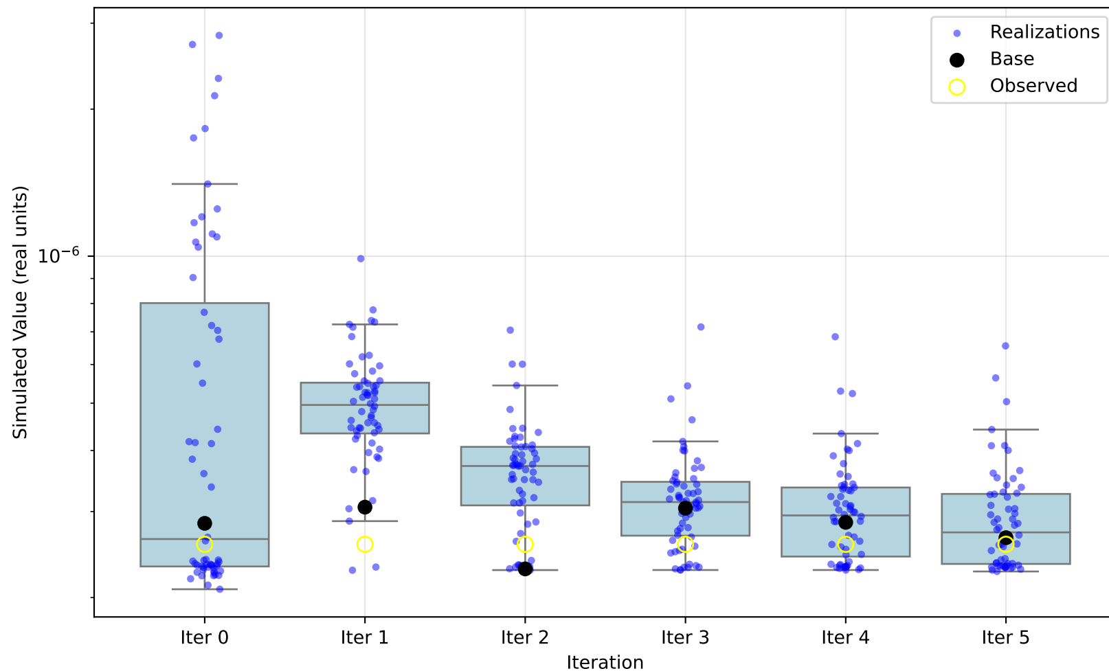
Simulated Ensemble vs Observed: mn
