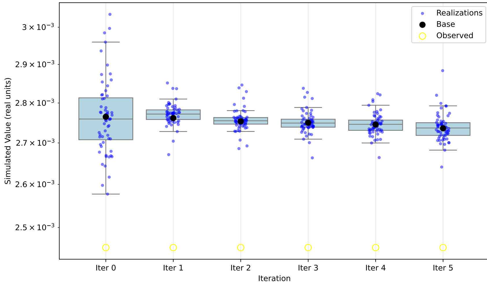
Simulated Ensemble vs Observed: na
