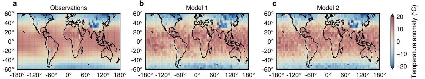
Figure 4. Generated toy data with independent noise per model. (a) Observations, near-surface air temperature anomalies in the time between 1980 and 2014 with respect to the global mean value of this time period. (b) M_1(s) = Y(s) + \mathcal{N}(0, 2) . (c) Predictions of model 2, analogous to model \mathcal{M}_1 , but with independently sampled noise.
