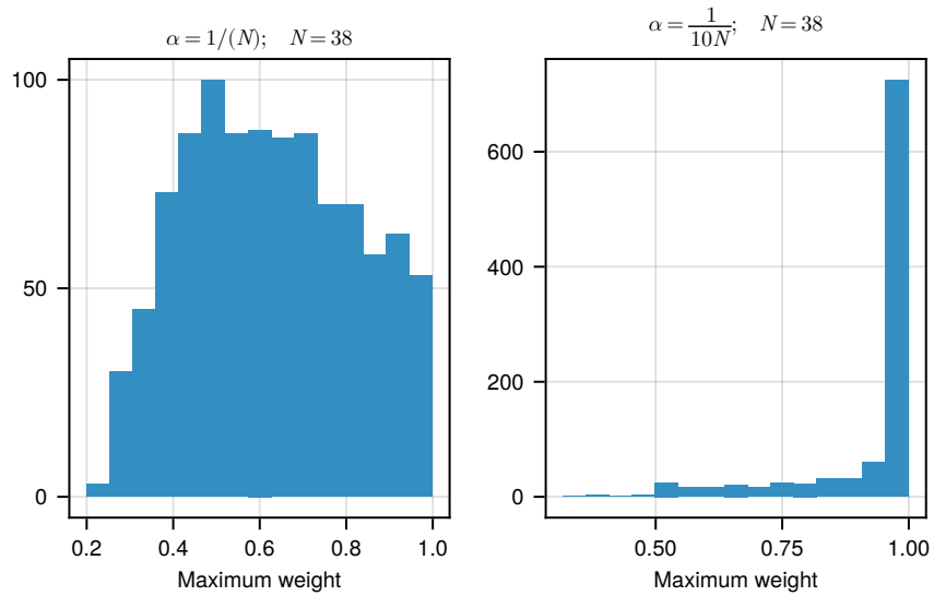
Figure C2. Histograms of the maximum element in each of 1000 vectors sampled from a Dirichlet distribution parameterized with \alpha = \frac{1}{38} (left) and \alpha = \frac{1}{380} (right).
