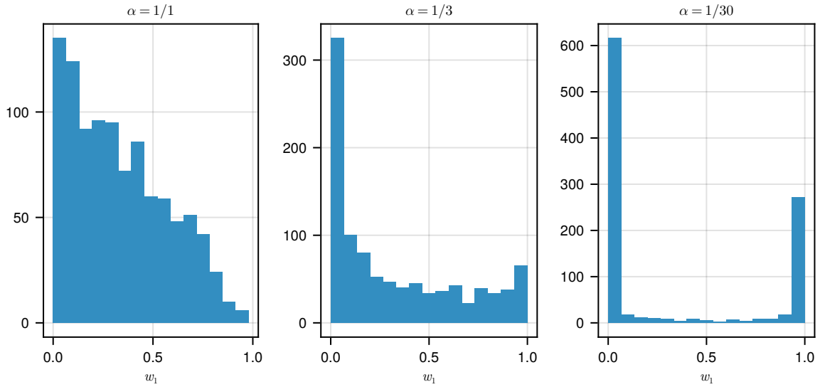
Figure C1. Histograms of the first element ( w_1 ) in 1000 vectors (of length 3) sampled from a Dirichlet distribution parameterized with different values of the concentration parameter \alpha .
