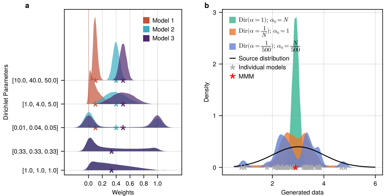
Figure 1. (a) Distributions of weights per model sampled from a Dirichlet distribution using different parameters. The stars show the mean weights. In the bottom two rows, the distributions of the individual model weights are identical, hiding the distributions for models 1 and 2 below the distribution for model 3. (b) Artificial data (grey dots) of 38 “models”, drawn from \mathcal{N}(\mu = 3, \sigma = 1) (black curve). The densities show the distributions of the expected data of the weighted average models computed for each of 10,000 weight vectors drawn from Dirichlet distributions with varying parameters.
