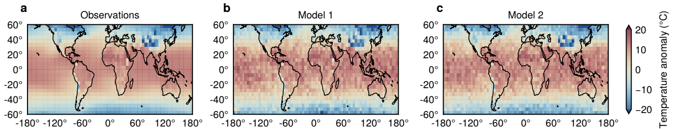
Figure 5. Observations of near-surface air temperature anomalies in the time between 1980 and 2014 with respect to the global mean value of this time period (a) and corresponding output of two real models, AWI-CM-1-1-MR (b) and CESM2-WACCM (c).
