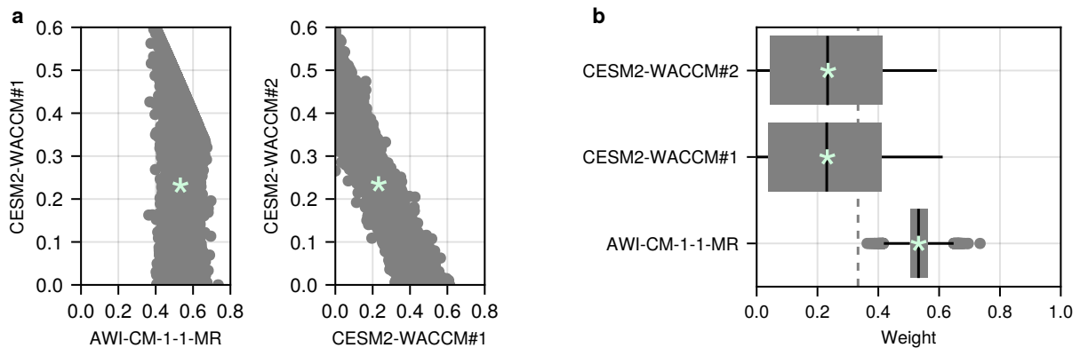
Figure 7. Posterior samples (showing the individual weights, i.e. the entries of the sampled weight vectors) using the ensemble performance weighting approach for a toy ensemble of 3 models and with Gaussian errors centered around 0; the variance is jointly sampled with the weight vectors. Green stars show the mean values (corresponding to values in Fig. 6f where n_2 = 2 ). The vertical dashed grey line in b indicates the value \frac{1}{N} = \frac{1}{3} .
