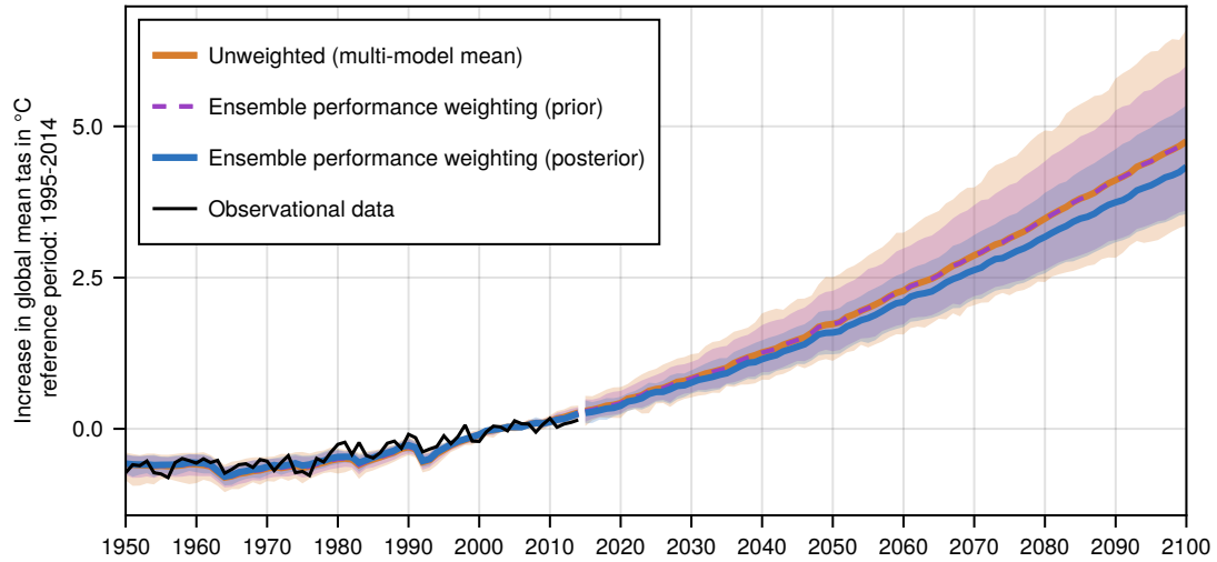
Figure 9. Projected increase in global mean near-surface air temperature with respect to the time period from 1995–2014 until the end of the century, under emission scenario SSP5-8.5, using an ensemble of N = 38 CMIP6 models. Thick lines show the observations (black), the multi-model mean (orange) and the weighted averages, using the mean posterior (blue) and mean prior (dashed purple) weights when applying the ensemble performance weighting approach with prior \text{Dirichlet}(\frac{1}{N}) and with the target distribution from Fig. 8 as likelihood. Uncertainty bands (shaded regions) represent the 0.05 and 0.95 quantiles of the predicted (weighted) ensemble spread.
