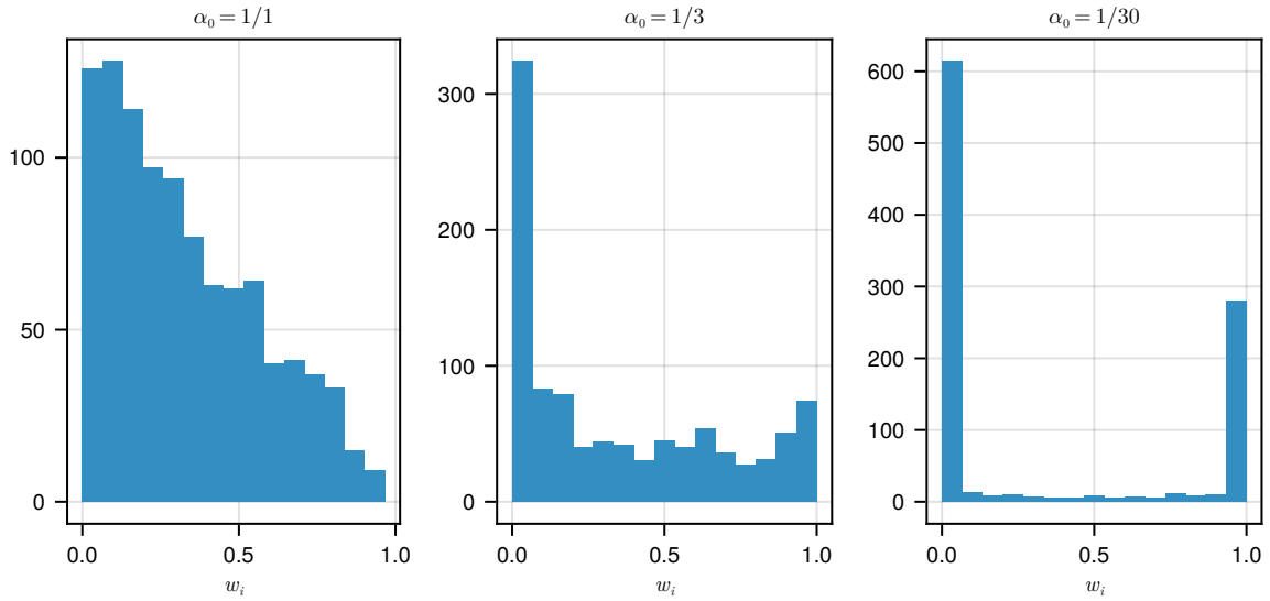
Figure C1. Histograms of the first element ( w_1 ) in 1000 vectors (of length 3) sampled from a Dirichlet distribution parameterized with different values of \alpha_0 .
