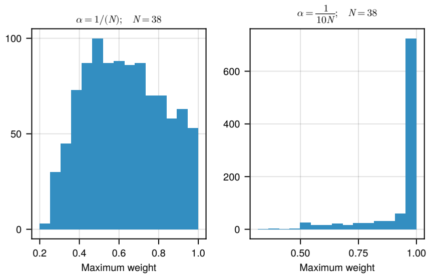
Figure C2. Histograms of the maximum element in each of 1000 vectors sampled from a Dirichlet distribution parameterized with \alpha_0 = \frac{1}{38} (left) and \alpha_0 = \frac{1}{380} (right).
