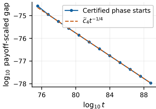
Order 4: phase-start gaps
