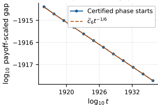
Order 6: phase-start gaps
