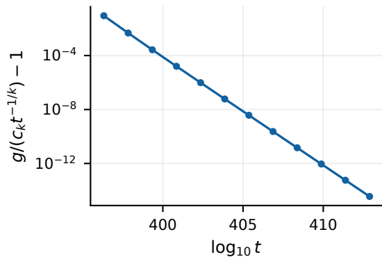
Relative error at phase starts
