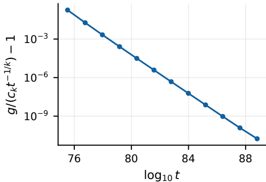
Relative error at phase starts
