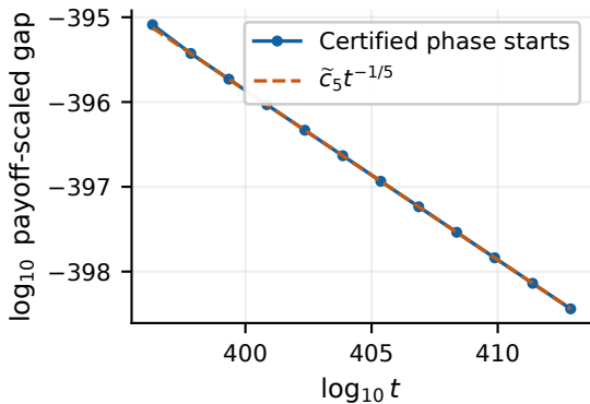
Order 5: phase-start gaps
