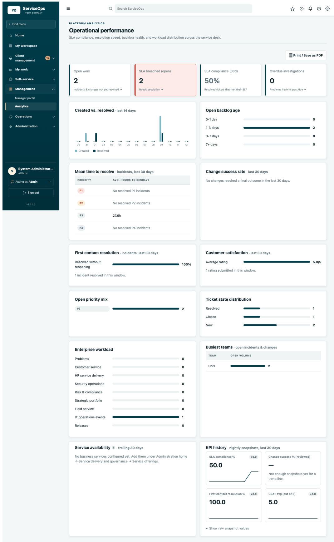
The analytics page: SLA compliance and breach/at-risk stat tiles, a 14-day created-vs-resolved trend chart, backlog aging buckets, mean-time-to-resolve by priority, change success rate, priority/state distribution bars, and a busiest-teams ranking.
