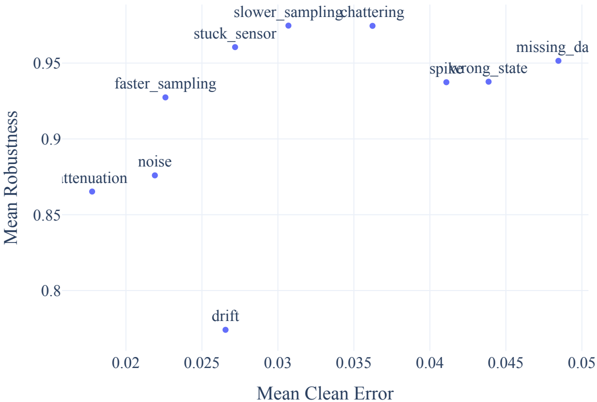
Mean Robustness vs. Clean Error for LSTM
