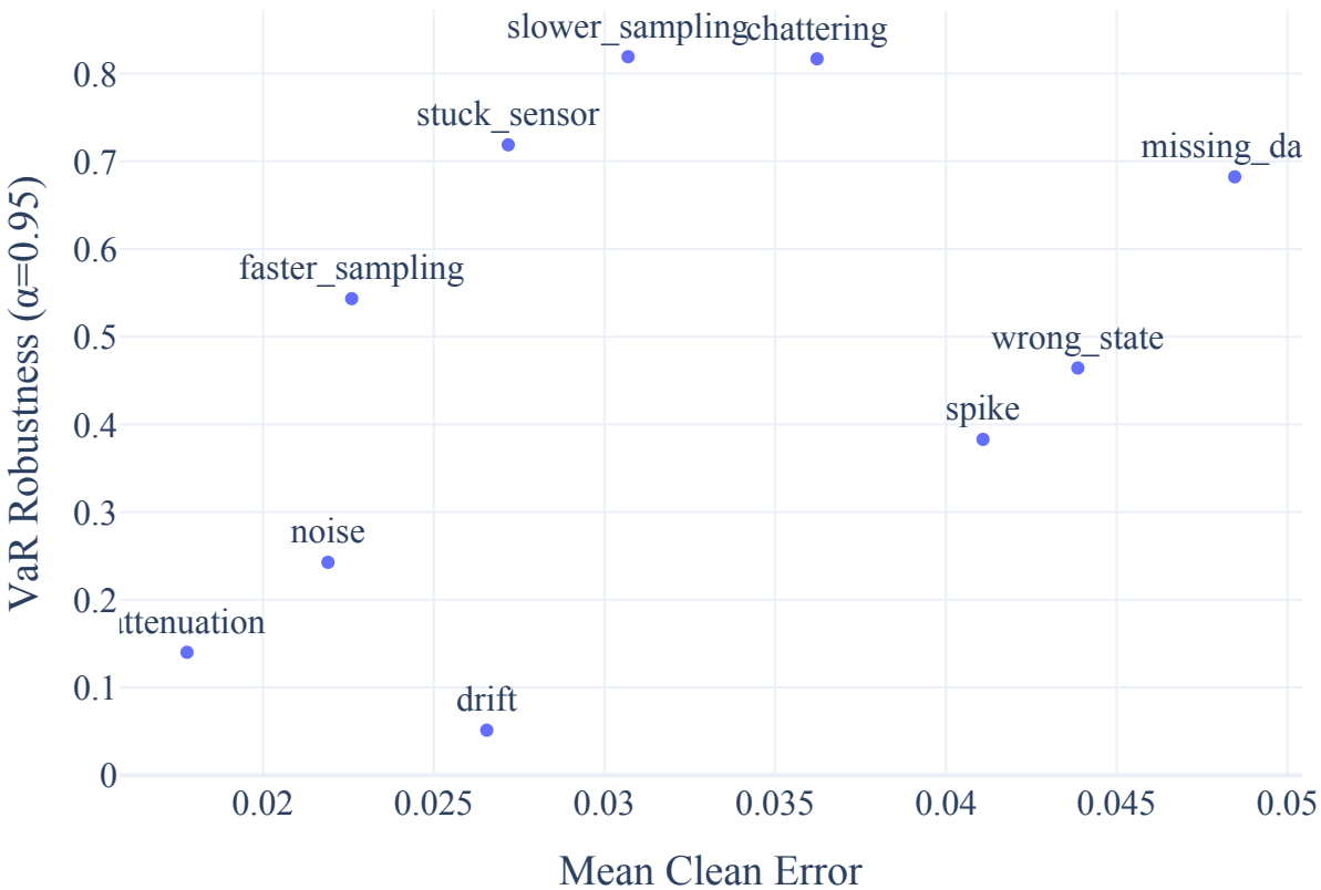
VaR Robustness ( \alpha=0.95 ) vs. Clean Error for LSTM
