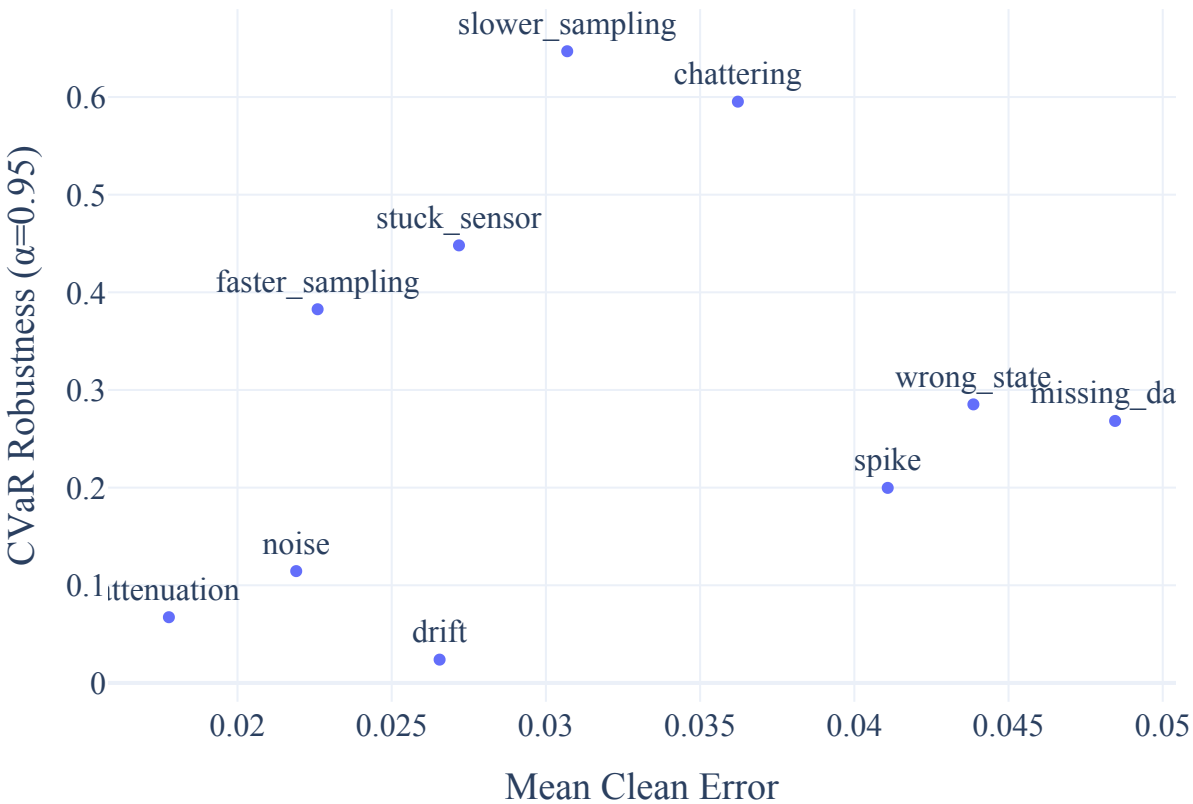
CVaR Robustness ( \alpha=0.95 ) vs. Clean Error for LSTM
