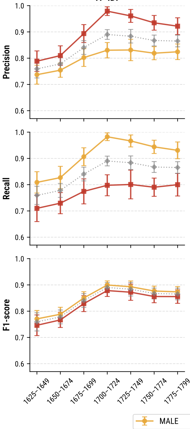
TF-IDF
