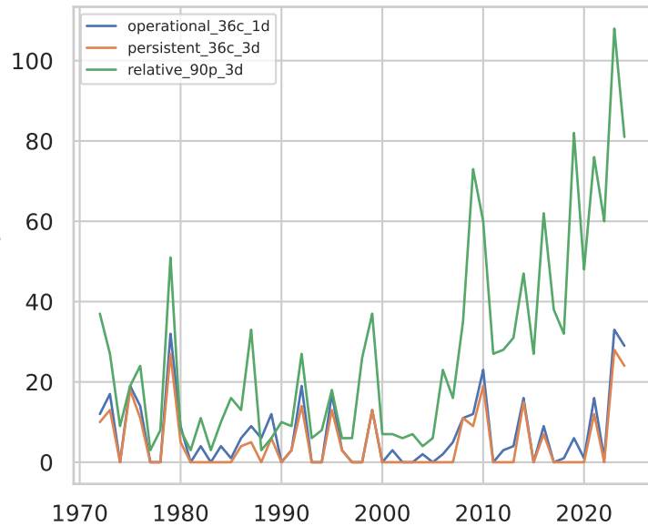
Heatwave-day frequency
