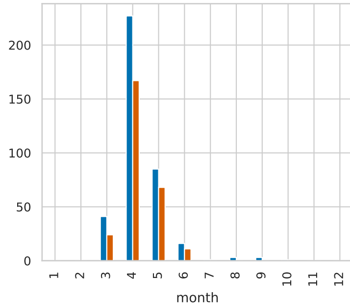
Monthly seasonality
