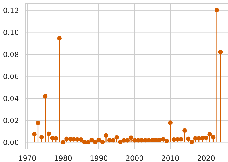
Cook's distance
