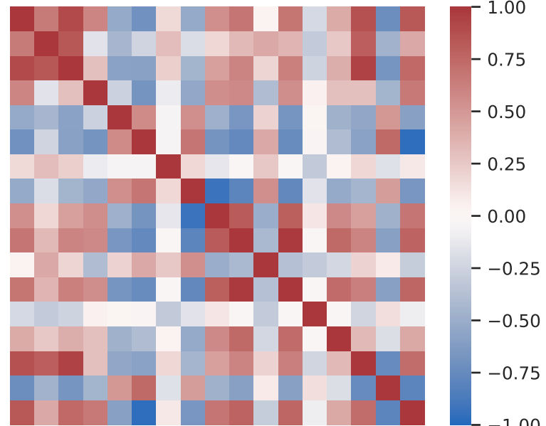
De-seasonalized correlations
