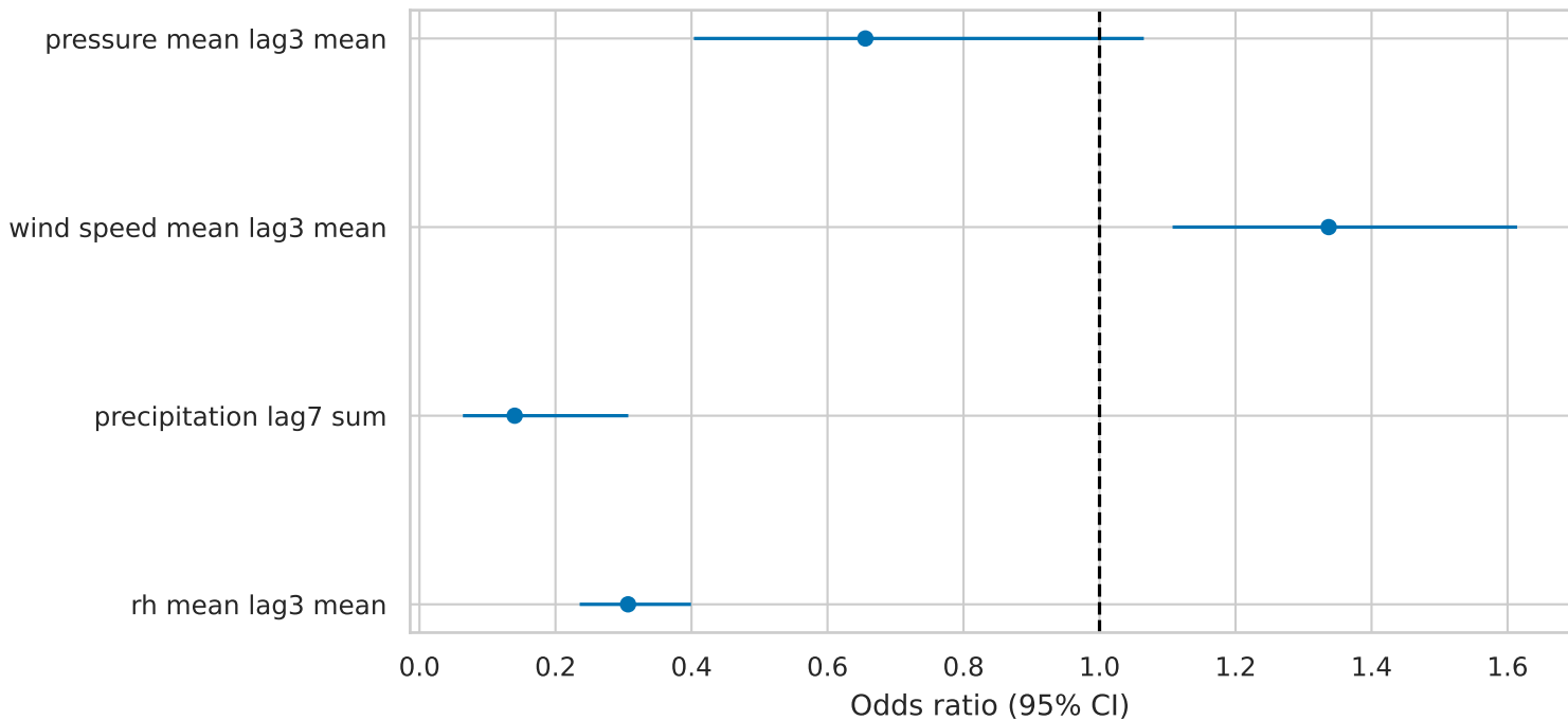
Adjusted antecedent associations (per SD)
