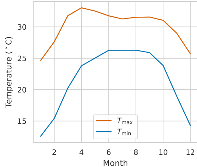
Monthly climatology
