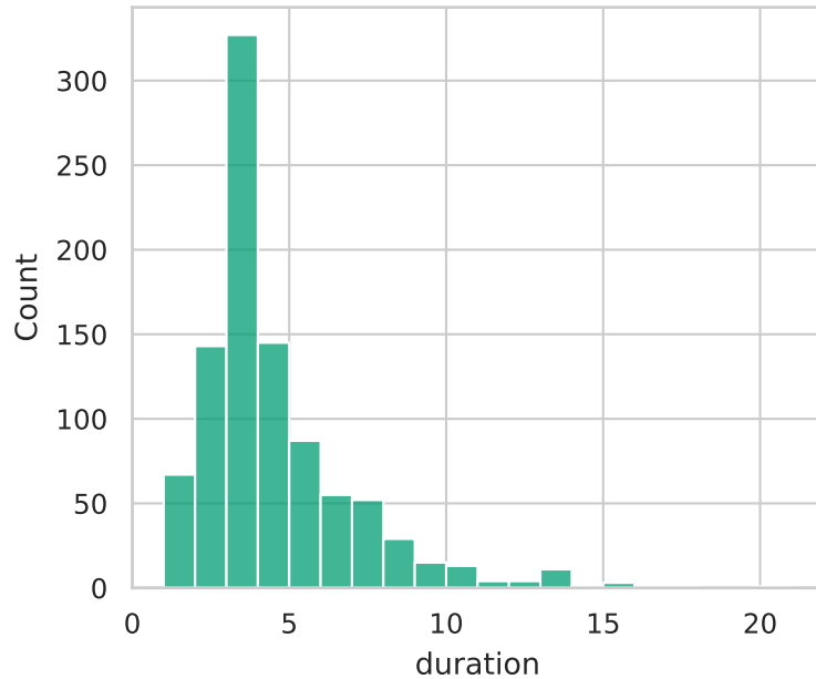
Event-duration distribution
