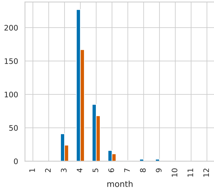
Monthly seasonality
