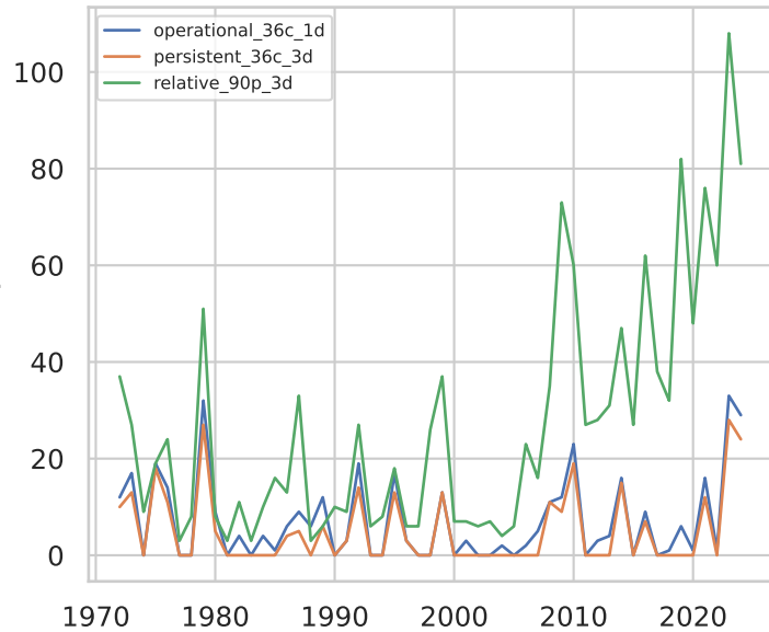
Heatwave-day frequency
