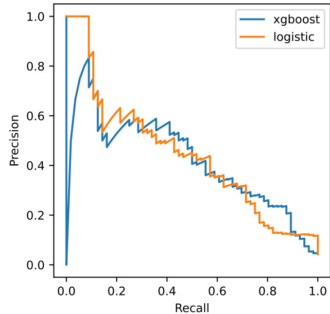
Pooled held-out precision-recall
