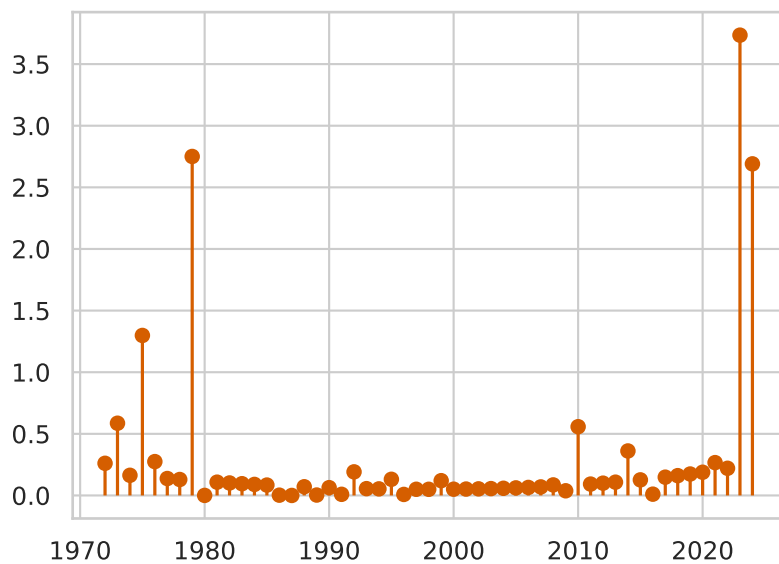
Cook's distance
