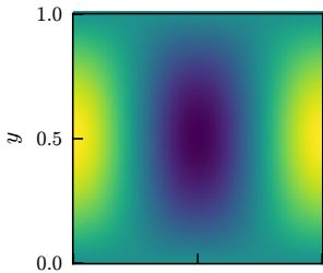
Exact u_x
