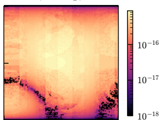
|u_x - u_x^*|
