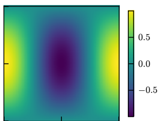
LiL u_x
