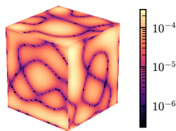
|w - w^*|
