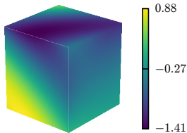
Exact v
