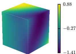
Exact p
