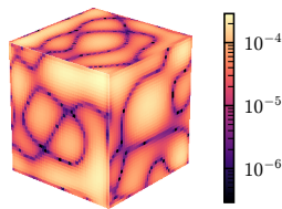
|v - v^*|
