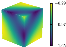
Exact p
